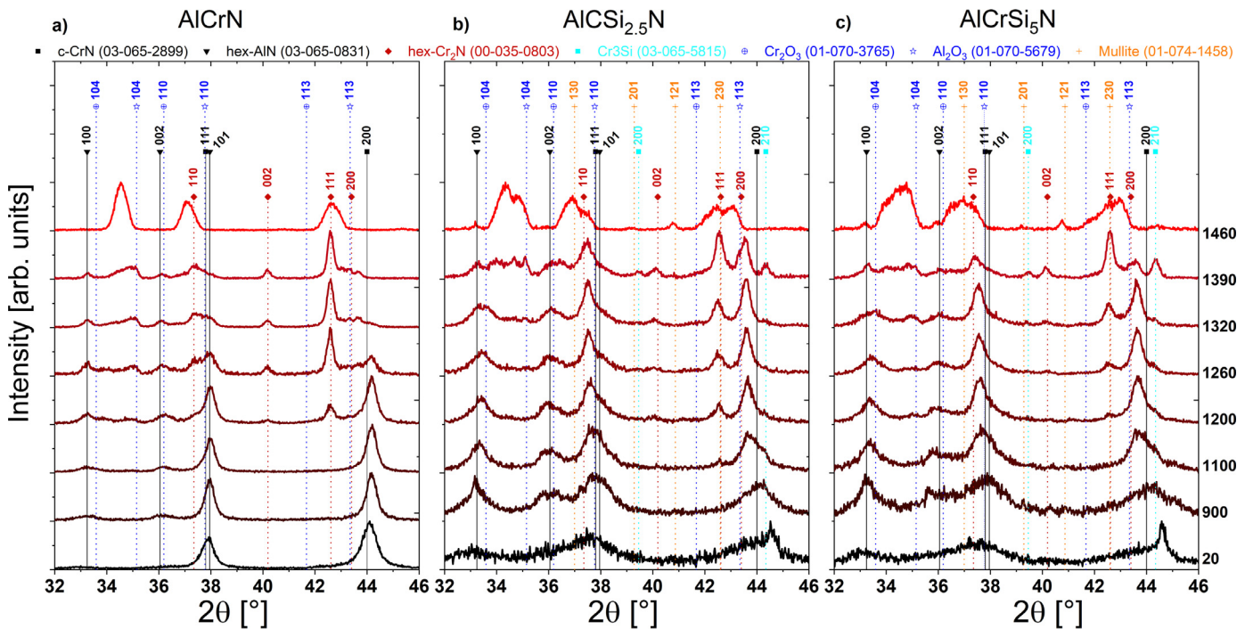
Fig. 3. X-ray diffractograms of (a) AlCrN, (b) AlCrSi 2.5 N and (c) AlCrSi 5 N coatings in the as-deposited state and after annealing at various temperatures in ambient air. Diffractograms with extended 2 angle are given in the supplementary Figure A.2 showing more details about the oxides formed in the Si-containing coatings after the DSC/TG experiment at 1460°C.
