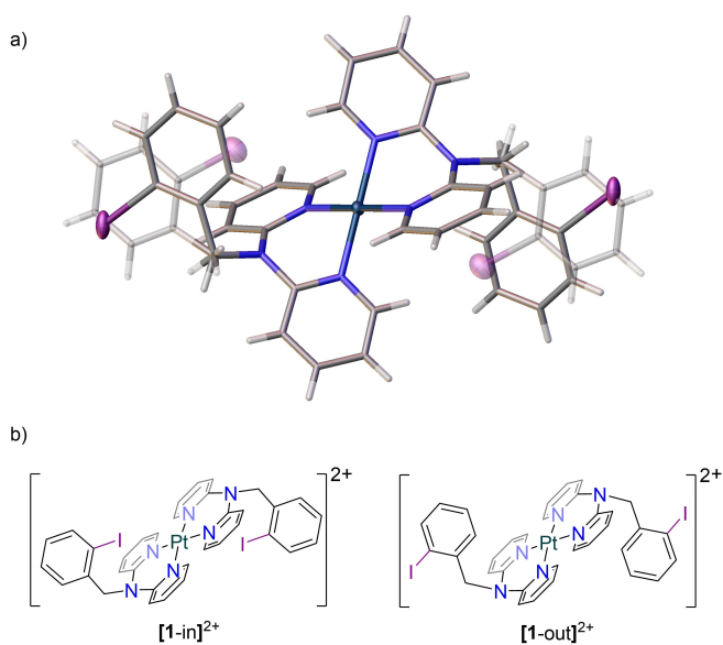
Figure 1. a) Disordered crystal structure of [1](OTf) 2 (the minor “in”-conformation is presented semi-transparently; triflate counterions are omitted for clarity), b) schematic drawing of [1-in] 2+ and [1-out] 2+ . [28]
