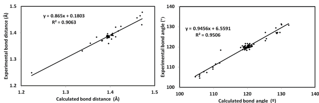
Figure 7. The correlations between the calculated and experimental geometric parameters.
