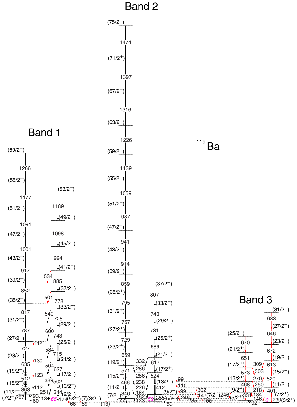
FIG. 1. Level scheme of ^{119}\text{Ba} . The new transitions are indicated with red, the bandhead energies of the three bands are indicated in pink, the isomeric and tentative levels are indicated with thick and dashed lines, respectively. The arrow widths are proportional to the transition intensities.
