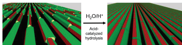
Figure 3. The proposed mechanism of CNC self-assembly within the native fiber template shown schematically.
