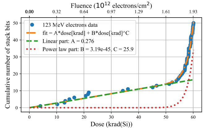
Fig. 3. Errors during irradiation with 123 MeV electrons at VESPER in memory SDF3. The figure shows the onset of new stuck bits in the memory as a function of the surface dose in Si and electron fluence. The trend of new errors has been shown with a fitted function, that is a sum of a linear part and a power law part. The fitting function is errors = A \cdot dose[krad(Si)] + B \cdot dose[krad(Si)]^C , where A , B and C are fitted parameters.
