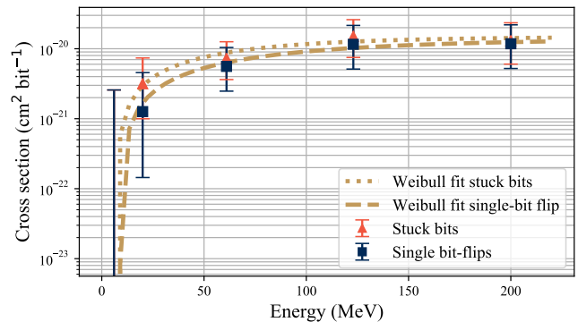
Fig. 6. Stuck bits and single bit-flip cross sections of electron irradiation under dynamic testing. The Weibull fits of the cross sections are also presented, which will be used later for a discussion of the memory behaviour in the Jovian environment. No events were observed for 6 MeV electrons, and only the upper limit is shown.
