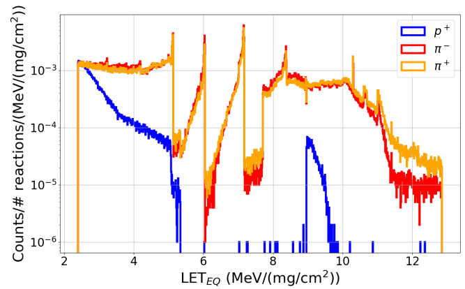
Fig. 16. Yield of secondary ions normalized to the number of interactions as a function of their LET_{EQ} for mono-energetic protons, negative pions and positive pions at 21 MeV.
