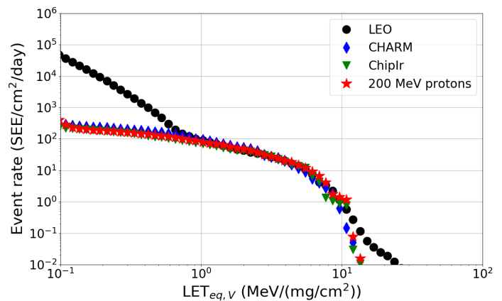
Fig. 5. Event rate normalized to a device surface of 1 \text{ cm}^2 per day for the LEO environment (800 km, 98^\circ , solar minimum, 100 mils of Al, trapped protons and galactic cosmic rays) compared with those from CHARM, ChipIr and 200 MeV protons scaled by the respective alpha factors. The volume considered for the Monte-Carlo calculations is typical of certain highly-scaled SEU structures.
