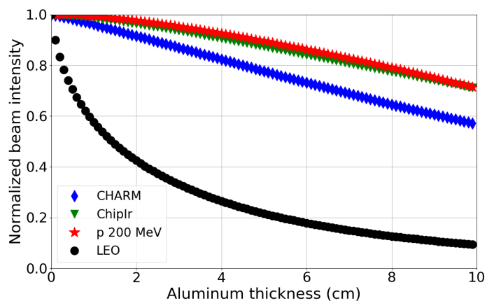
Fig. 3. Penetration depth of protons in Aluminium in the Low Earth Orbit proton environment compared to that of the mixed-field available at CHARM, that of spallation neutrons available at ChipIr and that from a 200 MeV mono-energetic proton beam. Only hadrons with energy above 20 MeV are considered for both space and facility environments.
