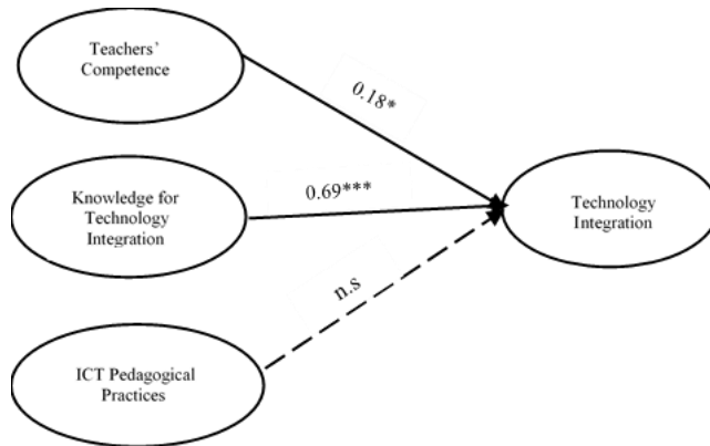
Fig. 1. The PLS-SEM Result of the Hypothesized Model.
