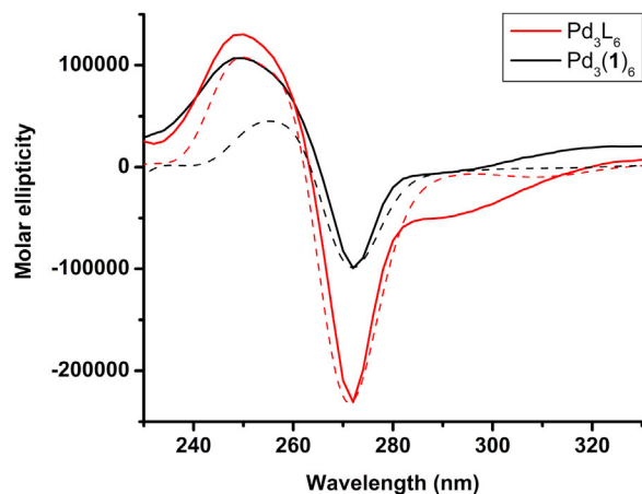
Figure 4. Electronic Circular Dichroism Spectra
