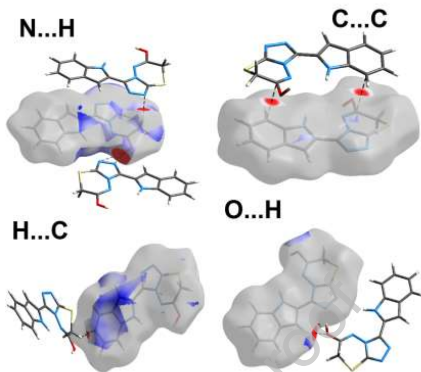
Figure 6. The d_{\text{norm}} maps of the most important intermolecular interactions in 2 .
