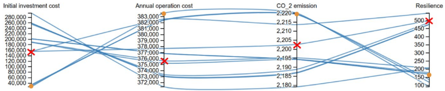
Fig. 5 Solutions after the third interaction of interactive K-RVEA. The orange dots are the aspiration levels forming the third reference point, and the red crosses are the aspiration levels forming the third reference point
