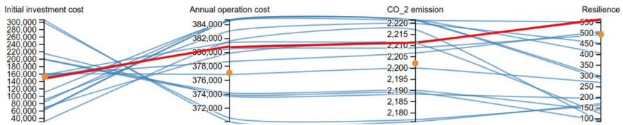
Fig. 6 Solutions after the fourth interaction of interactive K-RVEA. The orange dots are the aspiration levels forming the fourth reference point, and the red line is the most preferred solution selected by the DM
