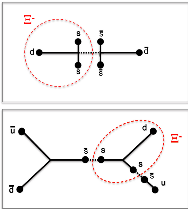
Fig. 9 Illustration of E^- production (top) in the standard Lund string framework, requiring diquark–anti-diquark pair production and (bottom) in a picture in which junctions are allowed to form
