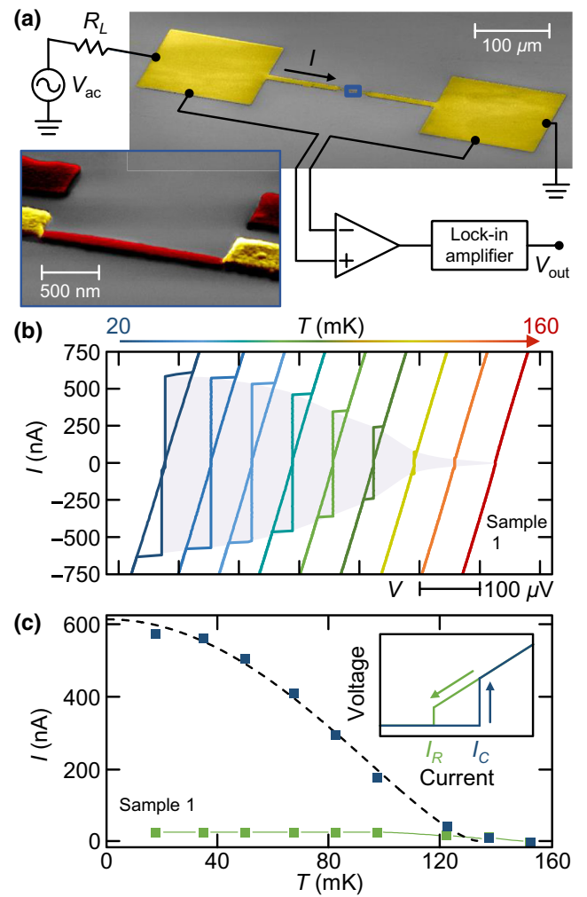
FIG. 2. Realization of the JES. (a) False-color scanning electron micrograph of a typical JES. The nanosensor is ac-biased (amplitude I ) and the voltage drop across the wire ( V_{\text{out}} ) is measured via a voltage preamplifier connected to a lock-in amplifier. R_L is a high-impedance load resistor. The inset shows an enlargement of the core of the JES showing the Al/Cu nanowire (red) in contact with thick Al leads (yellow). (b) Back-and-forth dc current-vs-voltage ( I - V ) characteristics of a typical JES measured at different temperatures T ranging from 20 to 160 mK in steps of approximately 20 mK. The curves are horizontally shifted for clarity. (c) Temperature evolution of the critical current ( I_C ; blue) and the retrapping current ( I_R ; green). The dashed black line is the critical-current prediction of the Bardeen model [43] (see the Appendix for details). The green line is a guide for the eye for the retrapping current. The inset shows the nanowire switches from the superconducting state to the normal state at I_C , while the transition from the resistive regime to the dissipationless regime occurs at I_R . The hysteretic behavior stems from Joule heating during transitioning from the normal state to the superconducting state [42]. I_R is almost temperature independent, and it is approximately 26.6 nA.
