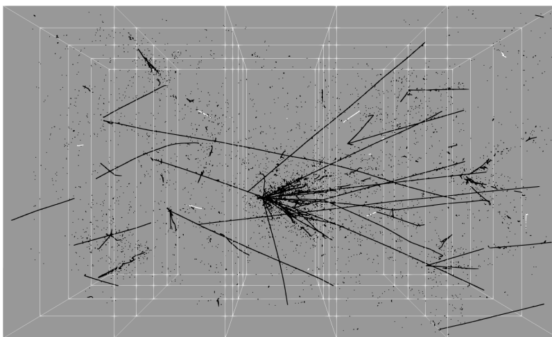
Figure A.13. A beam spill in the LAr component of the DUNE ND. The detector volume is 5 m × 4 m × 3 m. Fast-neutron induced recoiling proton tracks, with an energy threshold greater than ~ 10 MeV, are shown in white. The black tracks are all other energy deposits sufficient to cause charge collected at the pixel planes.
