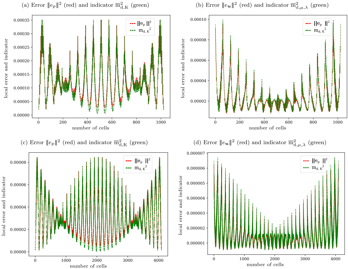
Fig. 1. Example 1 (Academic parameters). (a), (c) Local distribution of the error \|e_p\|^2 in red and the error indicator \overline{m}_{d,K}^2 generated by the majorant \overline{M}_p^h in green, and (b), (d) local distribution of the error \|e_u\|^2 in red and the error indicator \overline{m}_{d,\mu,\lambda}^2 generated by the majorant \overline{M}_u^h in green. The distributions are depicted w.r.t. numbered finite element cells of the uniform meshes with (a)–(b) h = 1/32 and (c)–(d) h = 1/64 . (For interpretation of the references to color in this figure legend, the reader is referred to the web version of this article.)
