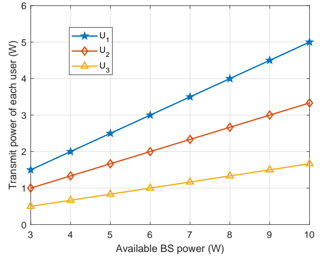
Figure 4. Available BS transmit power versus the power allocation of each user according to SIC constraint for M = 3 , PC = 1 , \beta = 1 .
