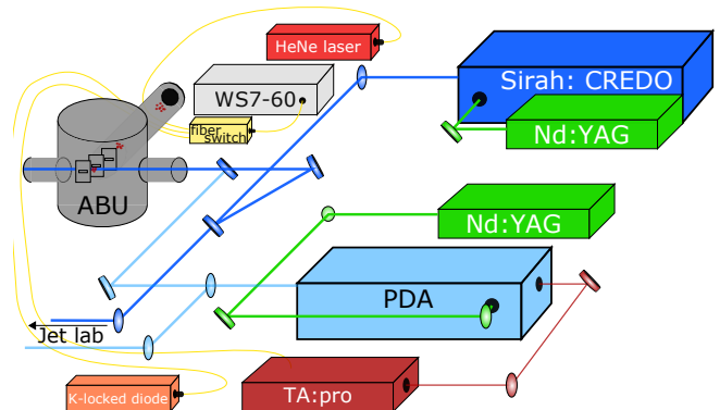
Figure 9: Schematic overview of the setup used to determine the hyperfine parameters of the 4s\ ^2S_{1/2} to 4p\ ^2P_{1/2} transition. For the in-gas-jet measurements, the UV laser beams were guided to the adjacent offline beam separator lab, see [15, 31].
