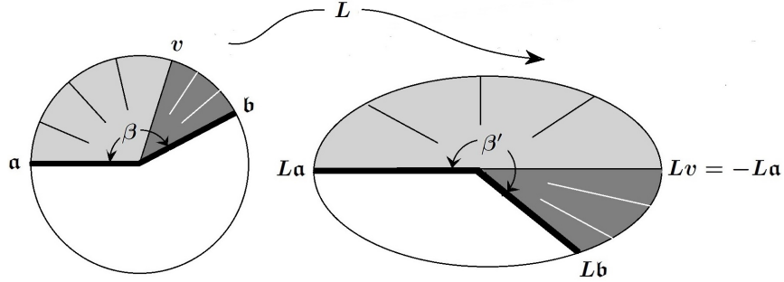
FIGURE 6. It is impossible to make 0 < \beta < \pi < \beta' < 2\pi by a linear transformation L: \mathbb{R}^2 \rightarrow \mathbb{R}^2 . Otherwise L would take two independent vectors \mathbf{a} and v into two linearly dependent vectors L\mathbf{a} and -L\mathbf{a} .
