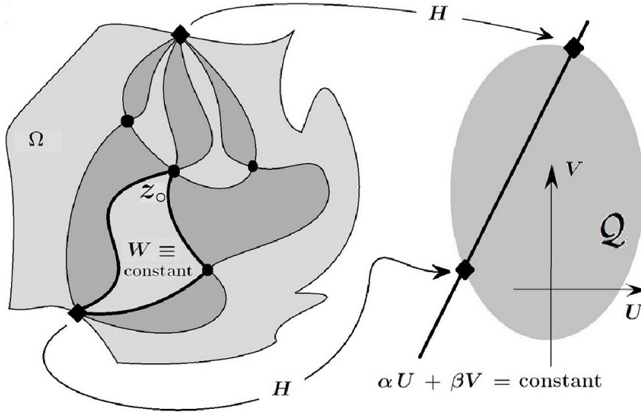
FIGURE 1. Kneser's proof of RKC-theorem in one drawing.
