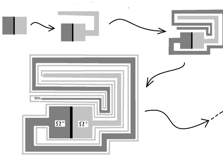
FIGURE 10. A nice straight line crosscut \mathcal{C} of a simply connected domain, \partial\Omega^- = \partial\Omega^+ = \mathcal{C} \cup \partial\Omega .
