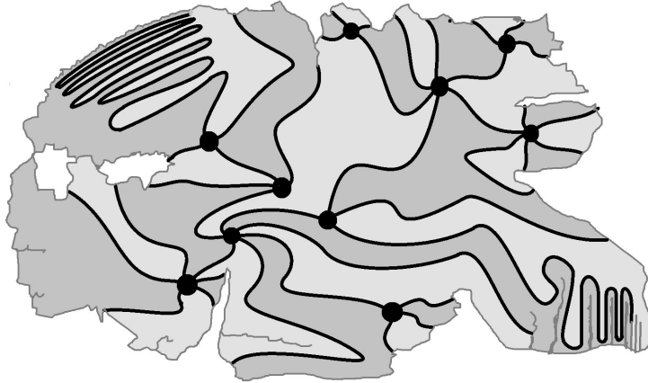
FIGURE 8. The shaded region marks a simply-connected domain \Omega \subset \mathbb{R}^2 . As we see, \Omega need not be the only complementary domain of \partial\Omega . Bullets are the critical points of u . The bold smooth open arcs are the level curves along which \nabla u \neq 0 . These arcs together with the critical points form what we call p-harmonic dendrite . The dendrite is locally connected and contains no simple closed Jordan curve. Every path along the dendrite that emanates from a critical point approaches the boundary of \Omega , possibly in a bizarre way.
