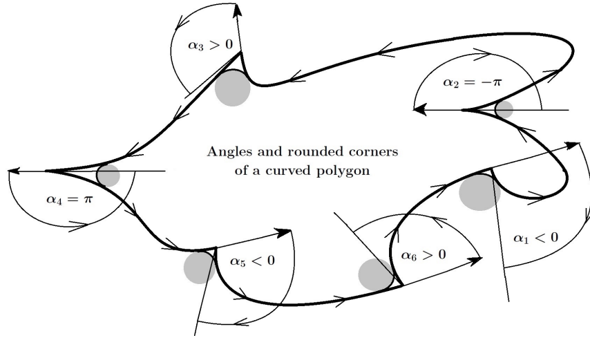
FIGURE 3. The circular arcs of small disks tangent to \Gamma . We replace the sharp corners of \Gamma by the circular arcs to form a \mathcal{C}^1 -smooth curve \Gamma^\varepsilon .
