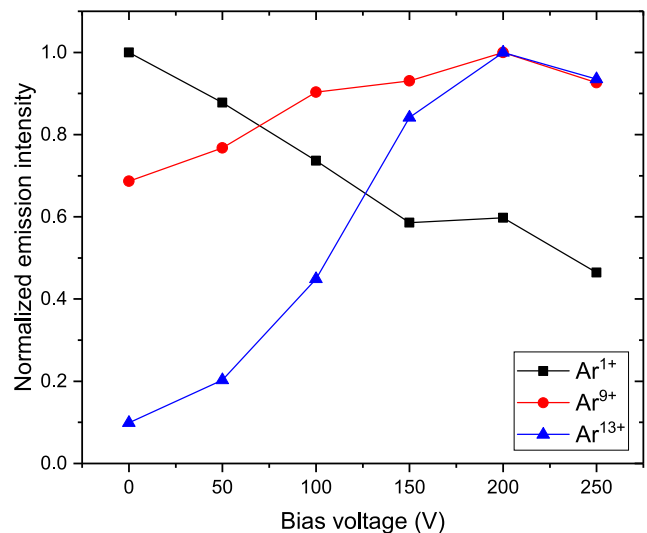
FIG. 2. The optical emission intensities of \text{Ar}^+ , \text{Ar}^{9+} , and \text{Ar}^{13+} as a function of the biased disc voltage (negative with respect to the plasma chamber).
