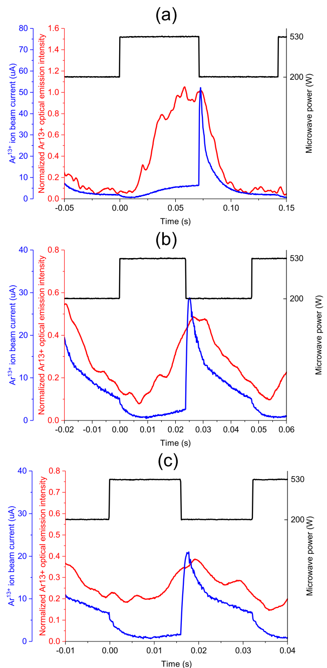
FIG. 3. The response of \text{Ar}^{13+} optical emission and beam current to amplitude modulation at (a) 7 Hz, (b) 21 Hz, and (c) 31 Hz with 50% duty factor. Notice that the axis scales change between the subfigures.
