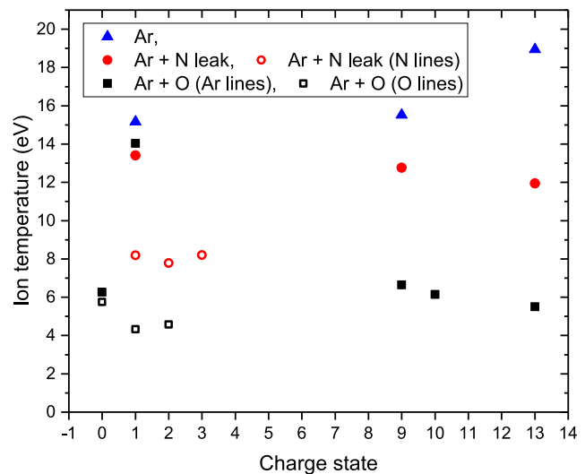
FIG. 4. The ion temperatures in discharges of pure argon, argon with a nitrogen leak, and argon with oxygen. In the first (Ar) and second (Ar + N 2 leak) case, the total pressure was optimized for Ar 13+ beam production, whereas in the last case (Ar + O 2 ) both, the total pressure and the gas mixing ratio were optimized for Ar 13+ beam production.
