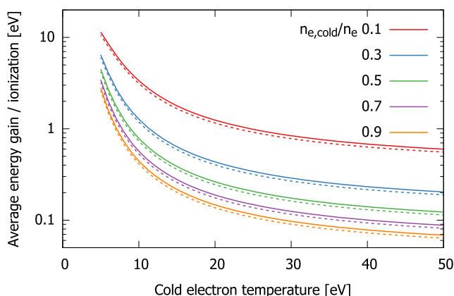
FIG. 7. The calculated average energy gain of the Ar^+ ion ionized via electron impact or charge exchange ionization as a function of the cold electron temperature at different cold electron fractions. The charge state distribution of the confined ions was taken either from afterglow peak currents (solid) or from continuously extracted currents (dashed).
