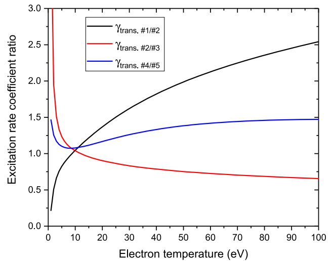
FIG. 6. Maxwellian rate coefficient ratios of the transitions suitable for determining the cold electron temperature in argon plasmas.
