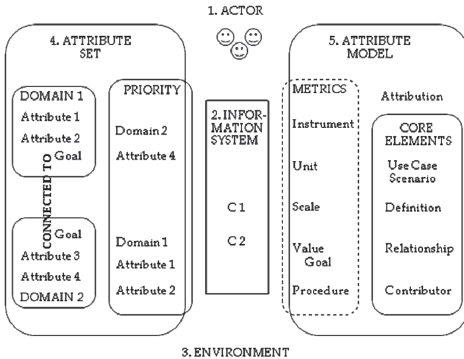
FIGURE 36 Intermediate version of quality meta-model
