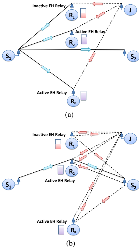
Fig. 17: Secure communication with untrusted relaying (a) DSHT (b) RDHT [266].
