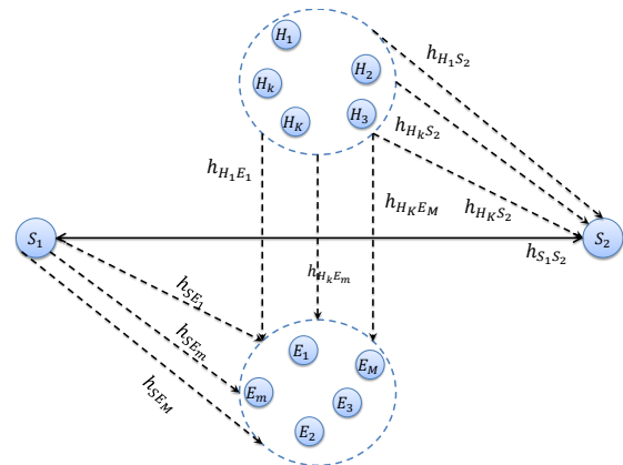
Fig. 3: System model.
