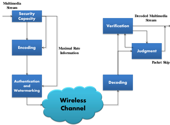
Fig. 15: Joint physical-application layer security scheme [204].
