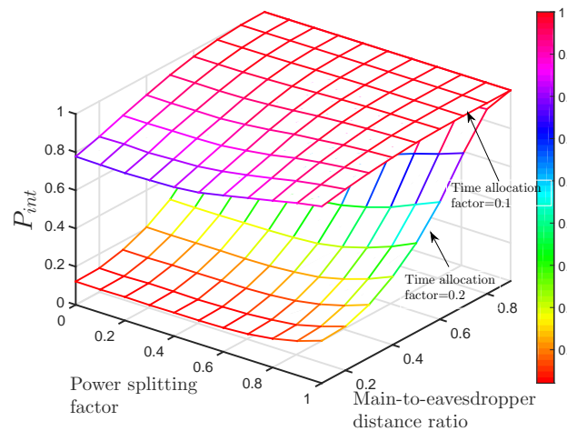
Fig. 20: Intercept probability against power splitting factor [110].
