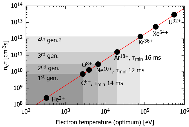
FIG. 2. The required product of n_e \tau at the optimum electron temperature to produce various fully stripped ions. The minimum ion confinement times of fully stripped C, Ne, and Ar ions displayed here correspond to the optimum electron temperature and critical density at 6.4, 14, and 28 GHz, representing the limits of the 1st–3rd generation sources. The data for the so-called Golovanivsky plot are taken from Ref. 1.
