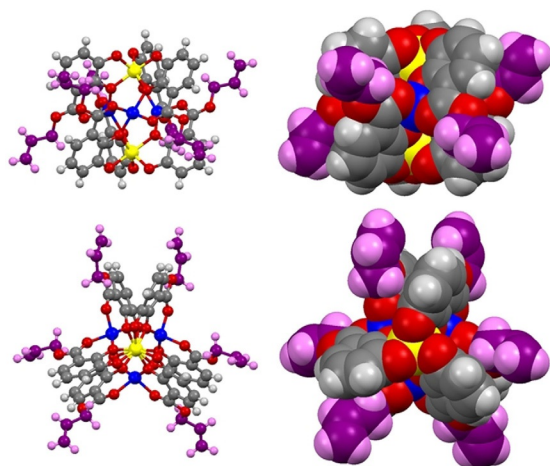
Figure 8. Structure of the anion [\text{Li}_3(\mathbf{2}^{\text{Al}}_3\text{Ti})]^- as found in the crystal. Top: "side view" (orthogonal to the Ti–Ti axis), bottom: "top view" down the Ti–Ti axis, left: ball and stick representation, right CPK representation. Yellow: Ti, blue: Li, grey: C, white: H, red: O, the allyl groups are shown in purple.
