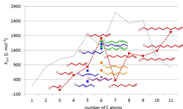
Figure 9. Dimerization constants of n -alkenyl derivatives [\text{Li}_3(\mathbf{2}_3\text{Ti})] in comparison to the corresponding n -alkyl esters (dotted blue line).
