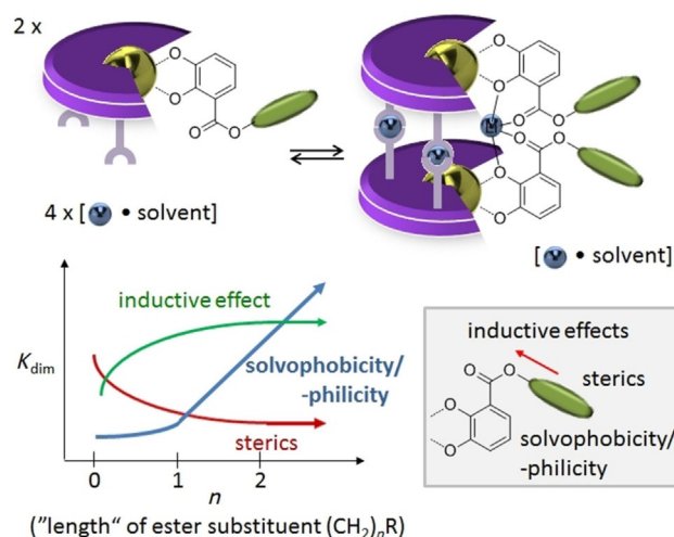
Figure 3. Different effects influencing the dimerization behavior to form hierarchically assembled helicates with hydrocarbyl ester substituted ligands in solution.
