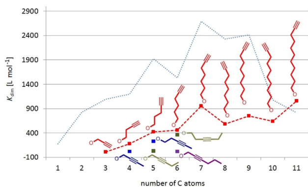
Figure 11. Dimerization constants in [\text{D}_6]\text{DMSO} of n -alkynyl derivatives \text{Li}[\text{Li}_3(3_n\text{Ti})_2] in comparison to the corresponding n -alkyl esters (blue dotted line).
