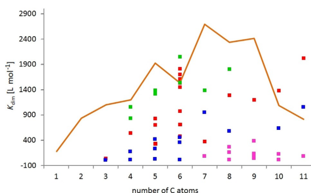
Figure 6. Distribution of the dimerization constants of primary hydrocarbyl substituted ester complexes \text{Li}[\text{Li}_3(\text{L}_3\text{Ti})_2] in [\text{D}_6]\text{DMSO} depending on the number of C-atoms of the substituent with branched alkyl (green), n -alkenyl (red), n -alkynyl (blue) and benzyl derivatives (magenta). The already reported data of the n -alkanes are used as standard and are shown as an orange line. [17]
