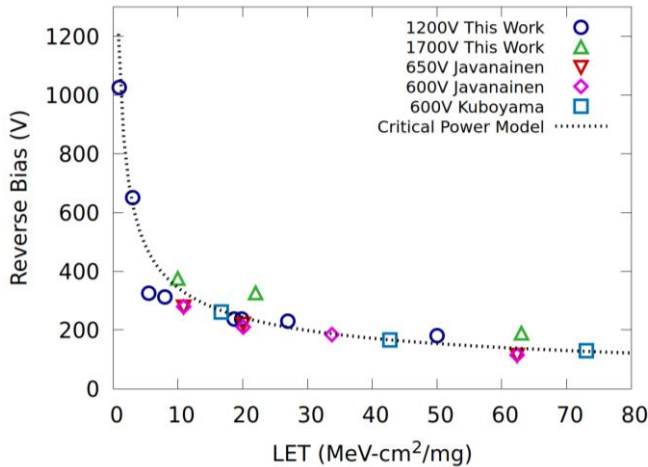
Fig. 1. Average observed reverse bias voltage thresholds for onset of heavy-ion-induced leakage current degradation in SiC JBS and Schottky diodes at various heavy ion LETs in silicon. New data from the experiments described here are included, as well as data from work done by Kuboyama et al. [13] and Javanainen et al. [14].
