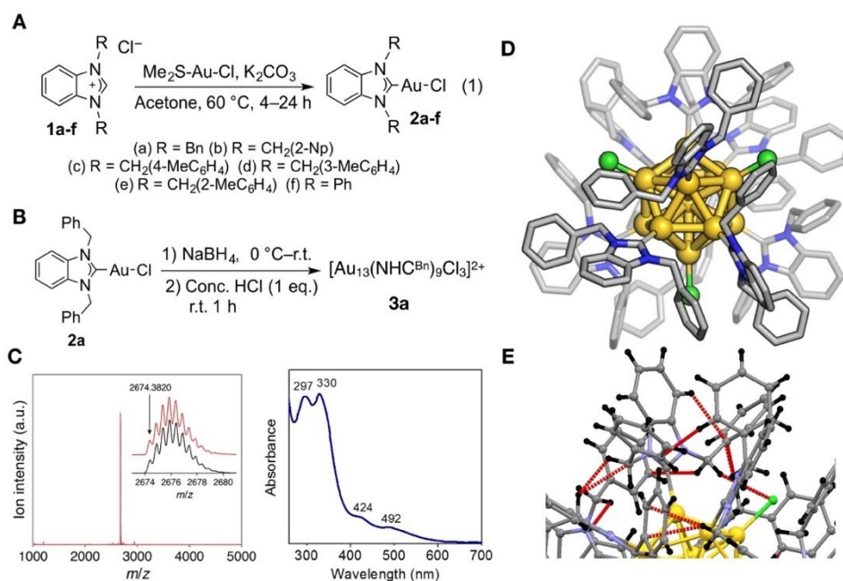
Fig. 2. Preparation and characterization of all-NHC Au 13 nanoclusters. (A) Synthesis of NHC–Au–Cl complexes as monomeric precursors for nanoclusters. (B) Optimized conditions for the synthesis of [Au 13 (NHC) 9 Cl 3 ] 2+ . (C) Characterization of nanoclusters by ESI-MS and UV-vis spectroscopy. (D) Single crystal X-ray crystallographically-determined structure of [Au 13 (NHC Bn ) 9 Cl 3 ] 2+ , (NHC = 1a ). Anions and hydrogen atoms have been removed, and wingtip phenyl rings shown as wireframe for clarity. Colour key: carbon (grey); nitrogen (blue); chlorine (green); gold (yellow). (E) Subset of inter-ligand CH–π interactions in 3a , showing the high degree of organization of the ligand shell.
