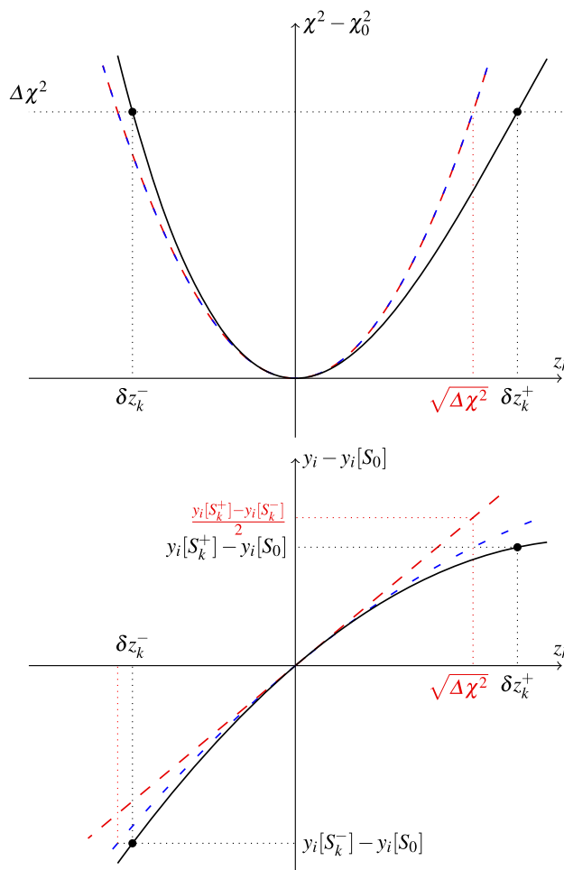
Fig. 1 An illustration for the response of \chi^2 (top) and y_i (bottom) with respect to a change of parameter z_k in quadratic-linear (red, long dashed), quadratic-quadratic (blue, short dashed) and cubic-quadratic (black, solid) approximations
