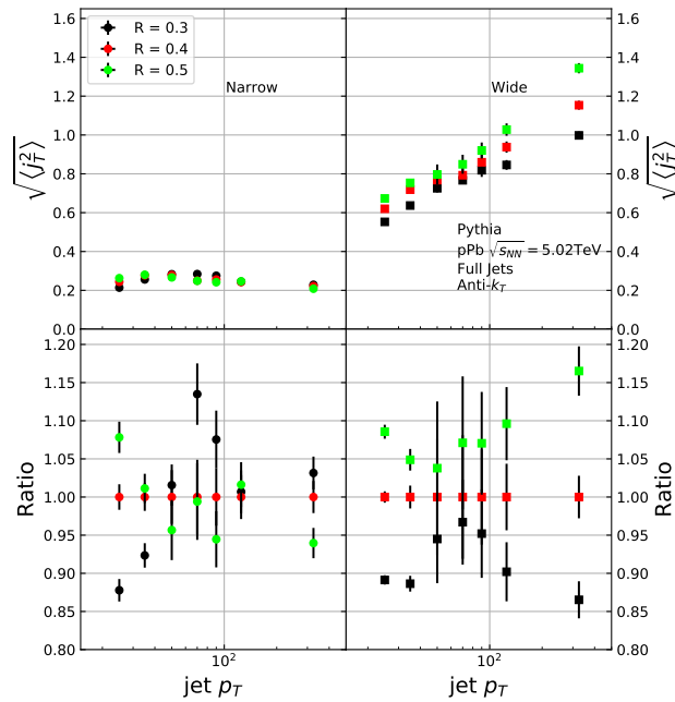
Figure 7.6: Effect of changing R parameter in jet finding on narrow and wide component RMS values. Wide component RMS values increase with increasing cone size.
