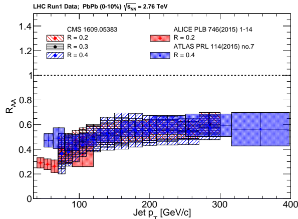
Figure 1.21: Reconstructed anti- k_T jet R_{AA} from ALICE [160] with R = 0.2 for |\eta| < 0.5 , ATLAS [161] with R = 0.4 for |\eta| < 2.1 , and CMS [162] with R = 0.2, 0.3 and 0.4 for |\eta| < 2.0 . The ALICE and CMS data are consistent within uncertainties while the ATLAS data are higher. The experiments use slightly different methods in selecting jets and subtracting the underlying event contribution. Compared to ALICE and CMS the ATLAS technique could impose a survivor bias and lead to a higher jet R_{AA} at low momenta as argued in [6]. Figure from [6].
