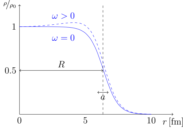
Figure 1.5: Woods-saxon distribution, with typical values for a Pb nucleus, a = 0.55\text{fm} and R = 6.6\text{fm} .
