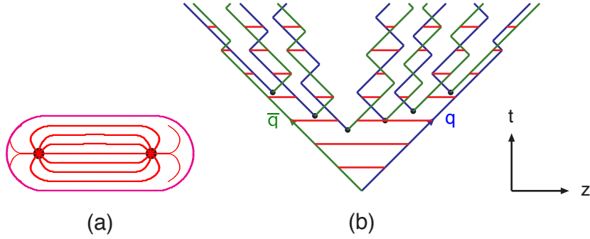
Figure 1.16: (a) A flux tube spanned between a quark and an antiquark. (b) The motion and breakup of a string system, with the two transverse degrees of freedom suppressed (diagonal lines are (anti)quarks, horizontal ones snapshots of the string field). This figure has been reprinted from [125] with kind permission from Elsevier.
