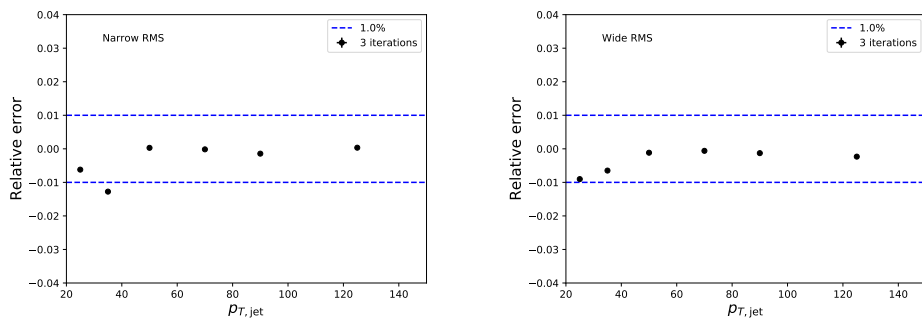
Figure 5.5: Unfolding with different number of iterations
