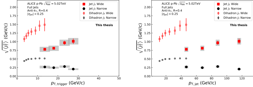
Figure 7.3: Jet j_T results are compared to results obtained in the dihadron analysis [277]. Dihadron trigger p_T bins are converted to jet p_T bins using observed mean p_{T,\text{jet}} values in p_{T,\text{trigger}} bins. Dihadron results are for 0.2 < x_{\parallel} < 0.4 .
