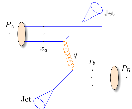
Figure 1.12: Schematic view of hard scattering process between two protons, producing two jets
