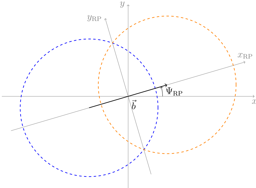
Figure 1.3: The definition of the impact parameter and the reaction plane. The x - y plane represents a coordinate system fixed by the experiment. The dashed circles are the two colliding nuclei. x_{RP} is the reaction plane and \Psi_{RP} gives its angle.
