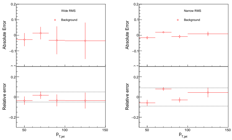
Figure 5.3: Differences between perpendicular cone and random background subtraction in the resulting RMS values
