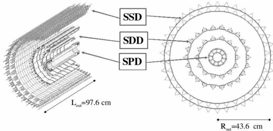
Figure 2.3: Schematic view of ALICE Inner Tracking System. Figure from [216].
