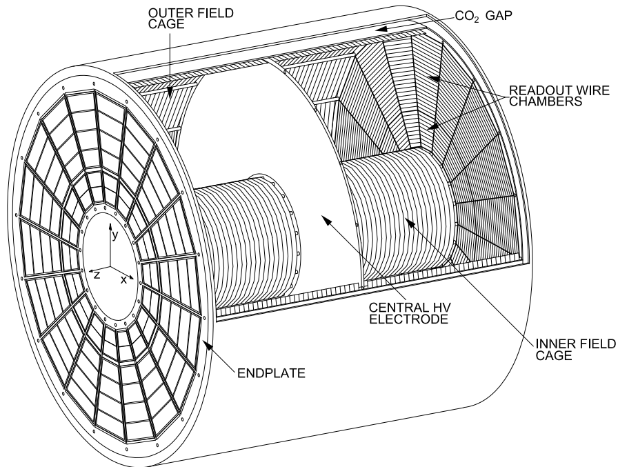
Figure 2.4: Schematic view of ALICE Time Projection Chamber. Figure from [231].
