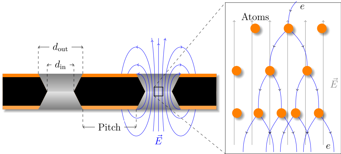
Figure 2.7: left Cross-section of a GEM foil. (Not to scale). The hole diameters are d_{\text{in}} = 50 \pm 5 \mu\text{m} and d_{\text{out}} = 70 \pm 5 \mu\text{m} and pitch is either 140 or 280 \mu\text{m} . right The amplification of a GEM foil is based on the Townsend avalanche phenomenon [258]. Electrons entering the electric field inside the hole are accelerated. If they gain enough energy before colliding with atoms they can liberate additional electrons, which are further accelerated leading to a chain reaction.
