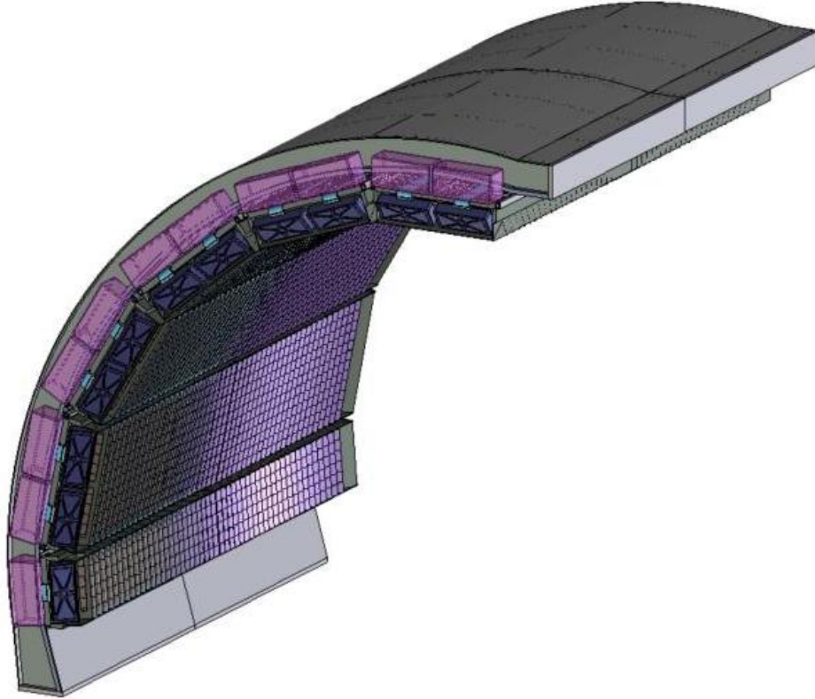
Figure 2.5: The EMCal detector arc, where the segmentation into 10 full size and 2 \frac{1}{3} -sized (5 and 1 per side) supermodules can be seen. Figure from [240]
