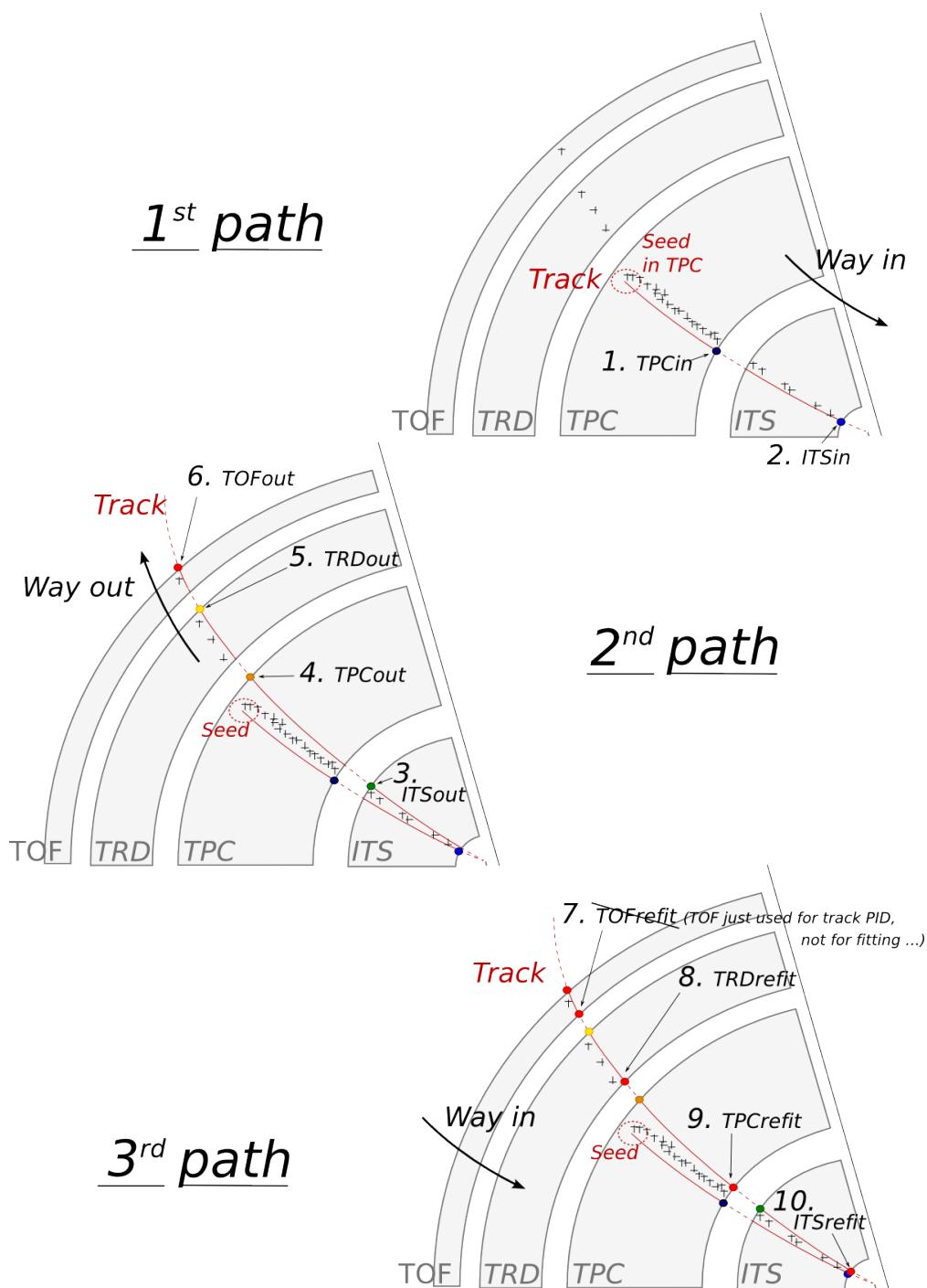
Figure 3.1: Principles of tracking in the ALICE experiment, showing the three successive paths allowing to build a track and refine its parameters. Numbers ranging from 1 to 10 mention the bits that are activated in case of success during the propagation of the Kalman filter at the considered stage. Figure from [265].
