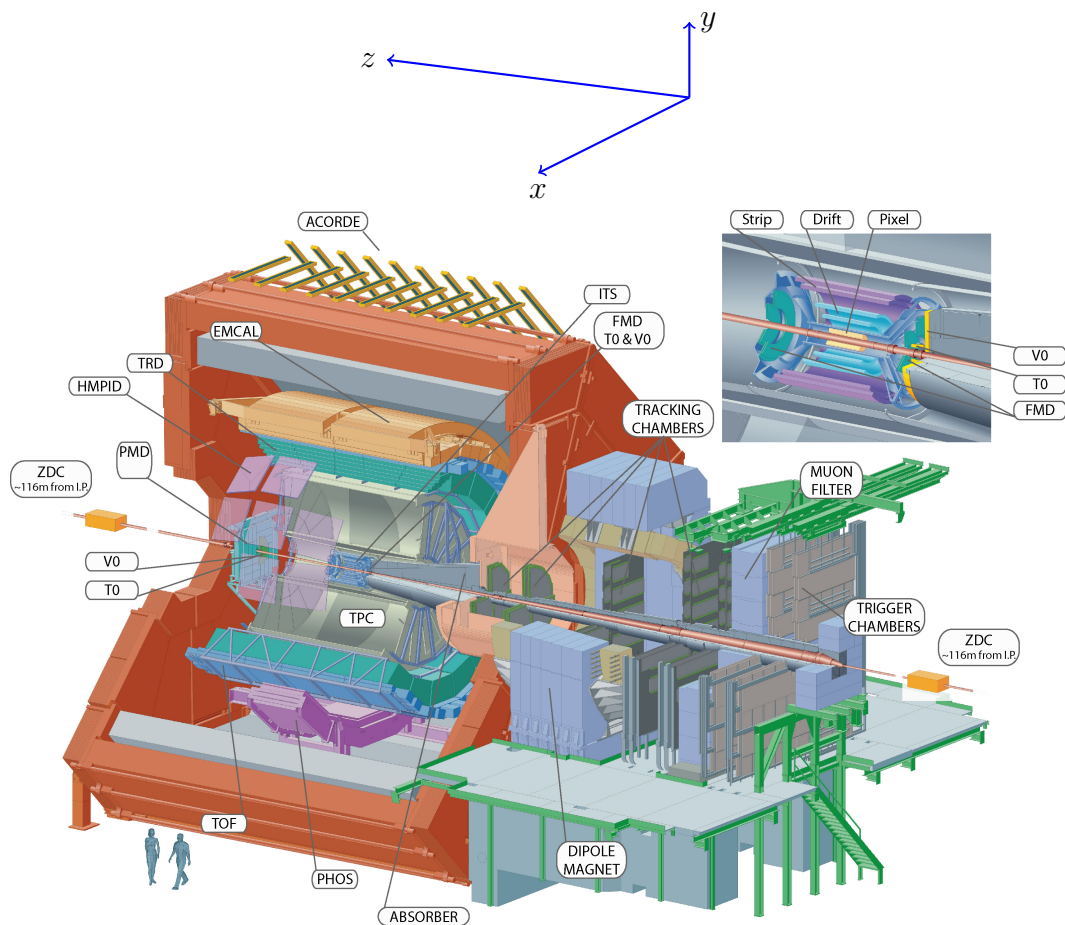
Figure 2.2: Schematic view of the ALICE detector with the definition of coordinates. The positive direction of z is also referred to as the A side and the negative direction as the C side.
