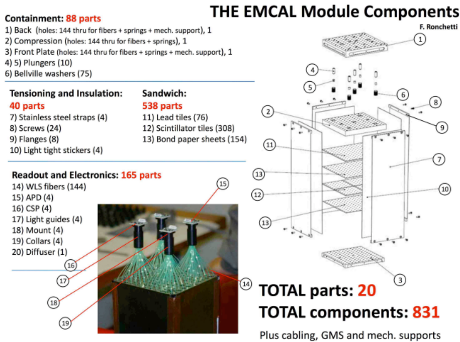
Figure 2.6: The exploded EMCAL tower view. Figure from [240].
