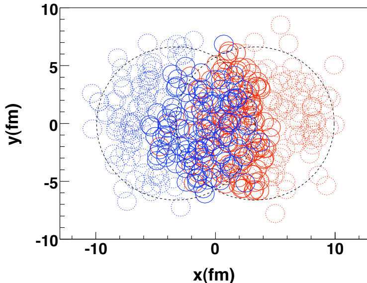
Figure 1.6: The figure shows a Pb–Pb collision in a Glauber Monte Carlo simulation. The big circles with black dotted boundaries outline the two colliding nuclei. Small blue and red circles represent nucleons with different colours for the two nuclei. Circles with solid boundaries are participants i.e. there is an overlap with at least one nucleon from the other nucleus. Circles with dotted boundaries are spectators which do not take part in the collision [89].
