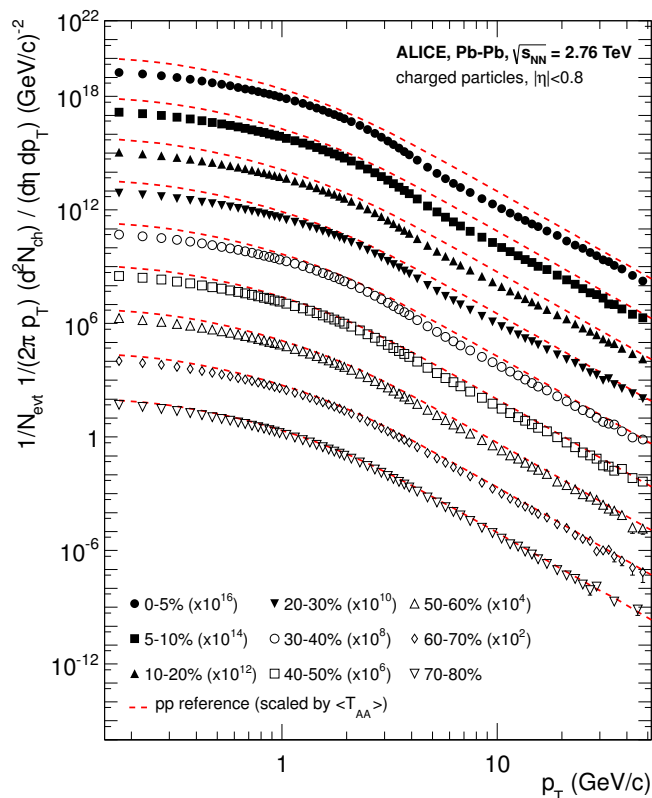
Figure 1.8: The radial flow is represented by the charged particle spectra for different centrality classes given in the legend. The dashed lines show proton-proton reference spectra which are scaled by the nuclear overlap function determined for each centrality class. For clarity the distributions and the reference spectra are offset by arbitrary factors. Figure from [91].
