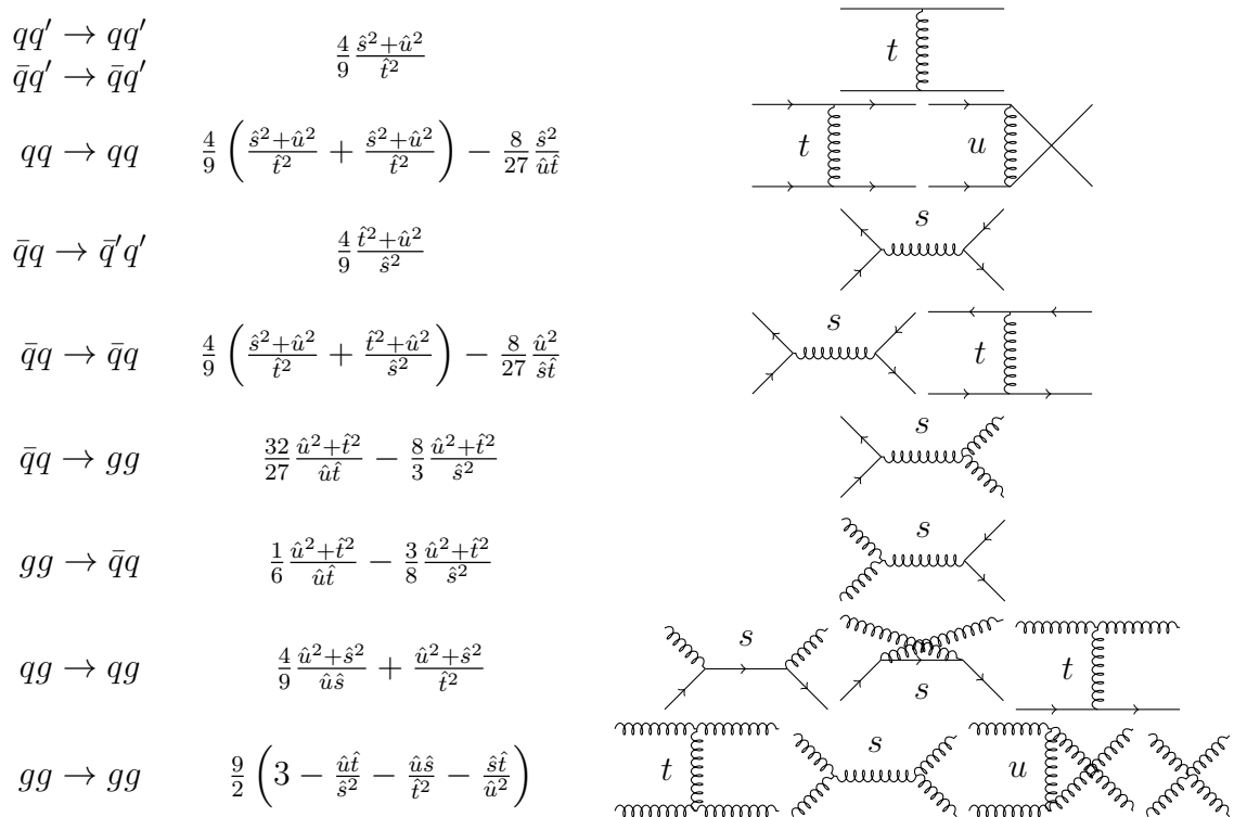
Figure 1.13: The basic pQCD processes and their quadratic matrix elements
