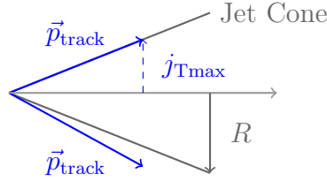
Figure 7.4: j_T has maximum value defined by the cone size and track momentum \vec{p}_{\text{track}}
