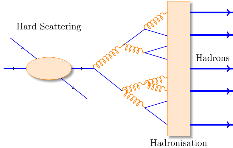
Figure 1.14: An illustration of jet showering. The highly virtual parton from the hard scattering will produce a shower of softer partons. When the virtuality is low enough the shower will go through a hadronisation process that produces the hadrons, which will be eventually observed in the detector.
