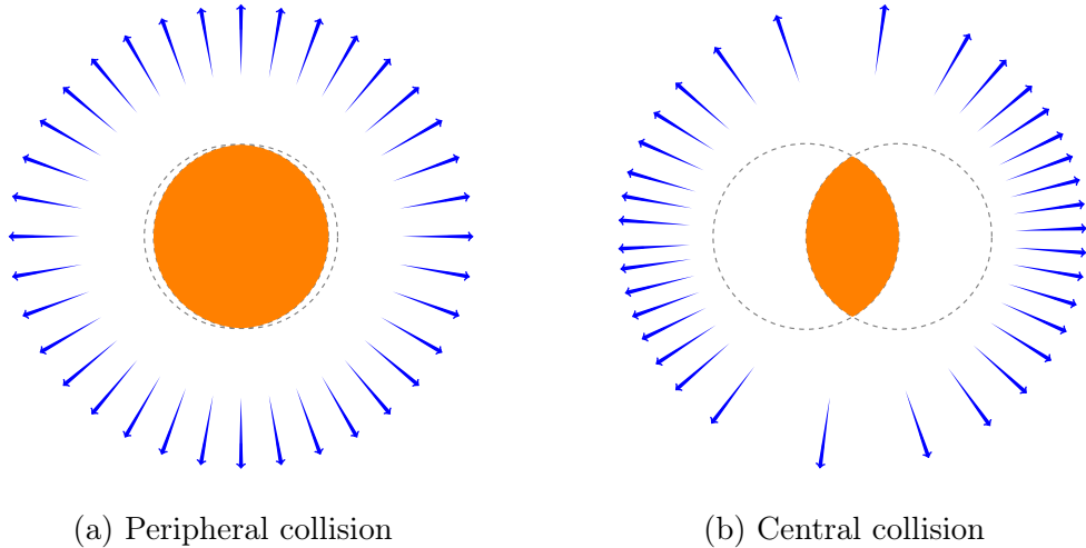
Figure 1.9: Illustration of elliptic flow in central and peripheral collisions. The density of the arrows represent the strength of flow in the corresponding azimuthal direction as seen in the detectors. In a peripheral collision momentum the difference in pressure gradients gives a strong flow into the in-plane direction while the flow into the out-of-plane direction is small. In a central collision flow is more isotropic and dominated by higher harmonics. In the figure the difference is exaggerated and the difference in total multiplicity is not taken into account.
