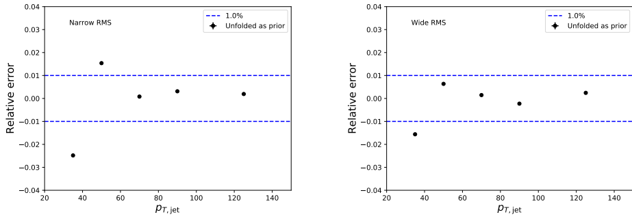
Figure 5.6: Effect of changing prior from true distribution in PYTHIA to the unfolded distribution
