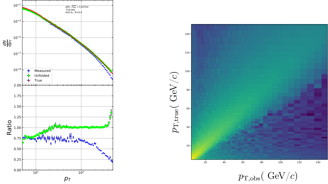
Figure 4.5: left : Unfolded jet p_T distribution in PYTHIA closure test right : Jet p_T response matrix from unfolding closure test
