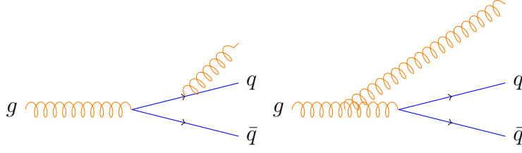
Figure 1.15: Soft gluon production
