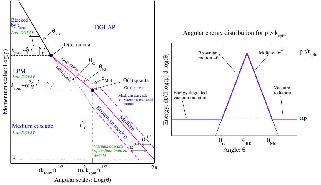
Figure 1.23: Left : Phase space view of dominant contributions in a medium-modified parton cascade. Right The distribution of energy as a function of angle for a fixed momentum with p > k_{\text{split}} . Large angular scales \theta > \theta_{\text{Mol}} are dominated by DGLAP vacuum radiation from the leading parton at the scale Q . At \theta < \theta_\alpha the energy density is dominated by vacuum radiation of the leading parton after it has degraded its energy propagating through the medium. Areas \theta_\alpha < \theta < \theta_{\text{BR}} and \theta_{\text{BR}} < \theta < \theta_{\text{Mol}} are dominated by Brownian motion and rare large angle (Molière) scatterings with medium partons. Figures from [165].
