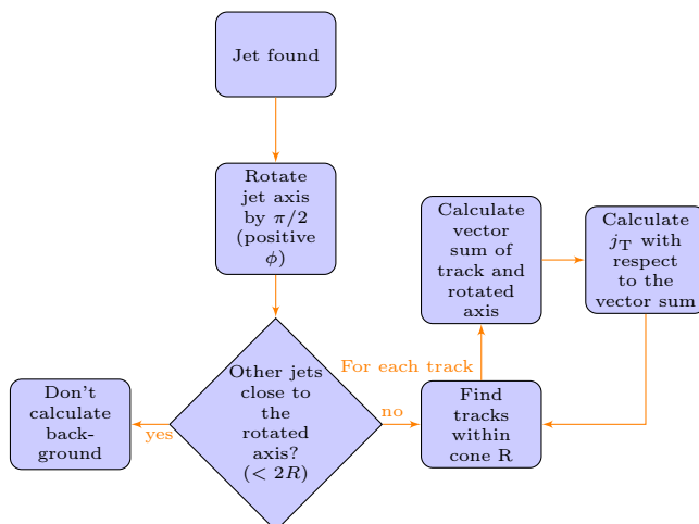
Figure 4.9: Flowchart representation of the perpendicular cone background procedure
