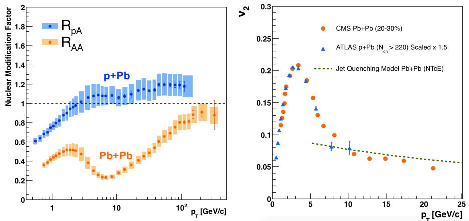
Figure 1.27: left : The nuclear modification factor R_{pA} in p–Pb collisions [193]. Compared to R_{AA} R_{pA} shows no sign of modification. right : The v_2 coefficient as a function of p_T in Pb–Pb and p–Pb collisions at the LHC [194, 198]. For shape comparison the p–Pb results have been scaled up by a factor 1.5. The green dotted curve [195] is a prediction from a jet quenching calculation where the anisotropy is driven by the directional dependence of the energy loss, rather than by hydrodynamic flow. This figure has been reprinted from [7] with kind permission from Annual Reviews.
