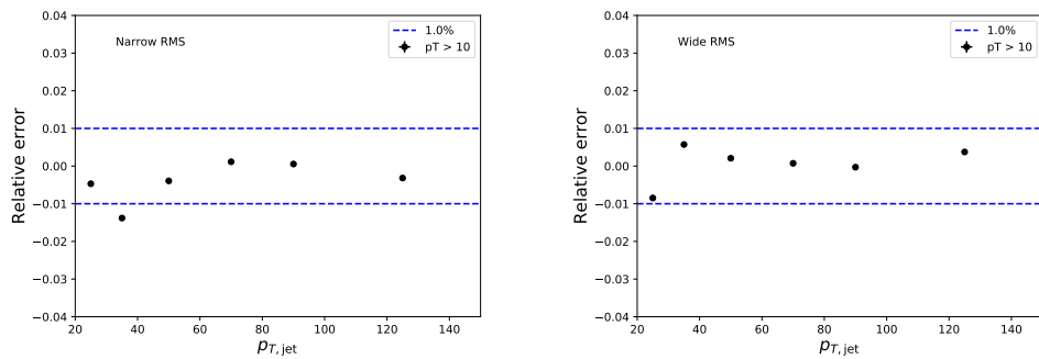
Figure 5.7: Effect of changing minimum jet p_T used in unfolding from 5 GeV/c to 10 GeV/c
