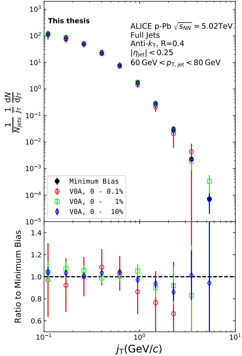
Figure 6.4: j_T distributions are shown for various multiplicity bins in p-Pb collisions.
