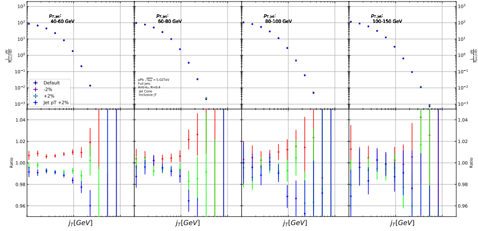
Figure 5.9: Results from PYTHIA simulations with Cluster energies scaled up and down by 2%. Additionally jet momenta were scaled by 2% when determining the jet p_T bin.
