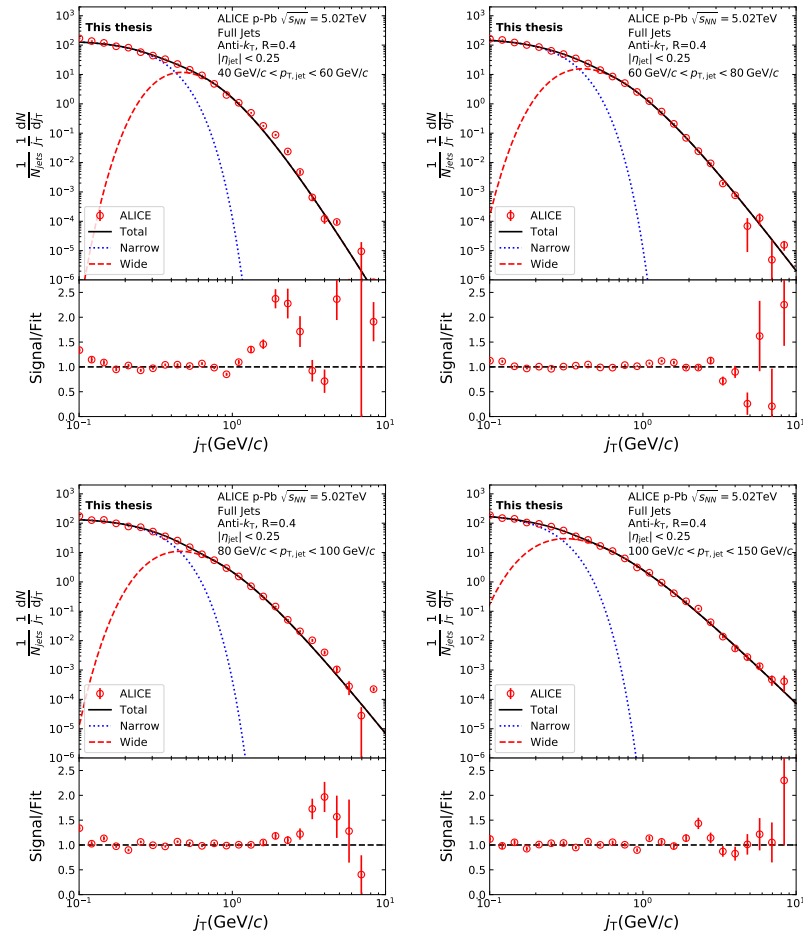
Figure B.1: j_T signal fits in different jet p_T bins
