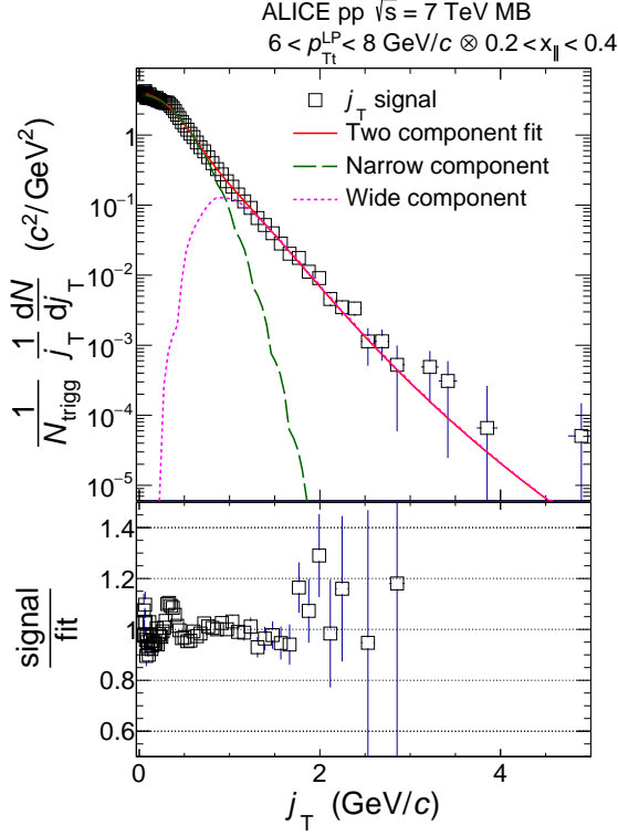
Figure 7.1: Measured j_T signal distribution using dihadron correlations is shown for 6 < p_{Tt} < 8 and 0.2 < x_{\parallel} < 0.4 . The distribution is fitted with the same two component model used in this thesis. Figure from [277].
