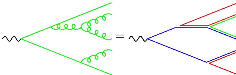
Figure 1.17: Colour structure of a parton shower to leading order in N_c . This figure has been reprinted from [125] with kind permission from Elsevier.
