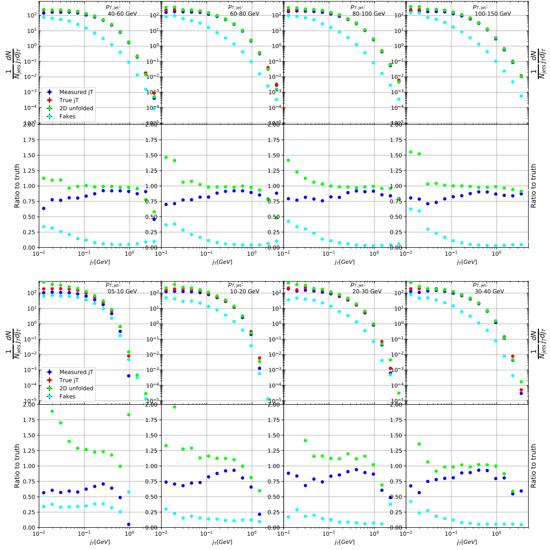
Figure 4.7: Pythia closure test results. Fake tracks include also tracks that do exist in the true dataset, but for one reason or another were not given j_T values. j_T is only calculated for tracks that are associated with jets.
