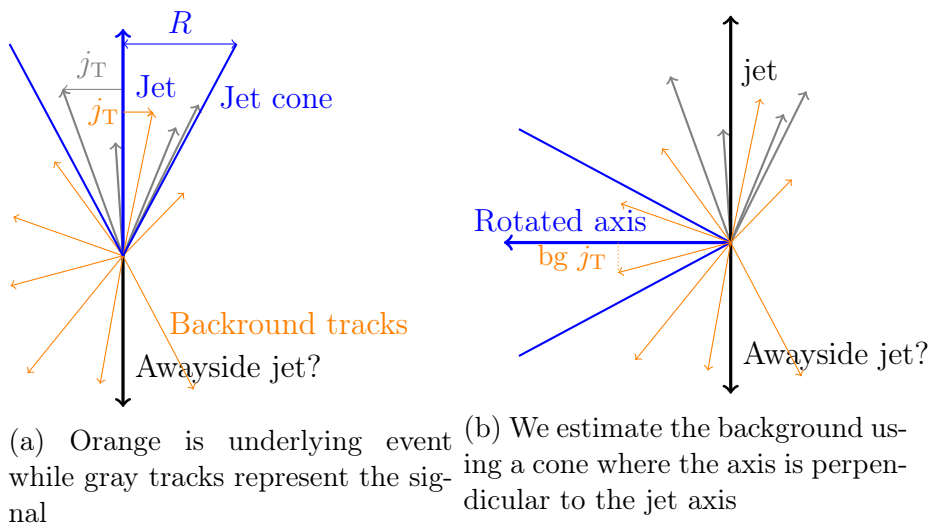
Figure 4.8: Background estimation
