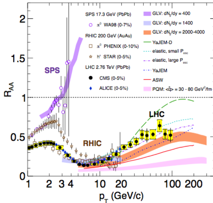
Figure 1.19: Measurements of the nuclear modification factor R_{AA} as a function of p_T in central heavy-ion collisions at three different centre-of-mass energies. Separate results are shown for different particle species [129–134] and the results are compared to predictions from several theoretical calculations [69, 135–139]. Figure from [134].
