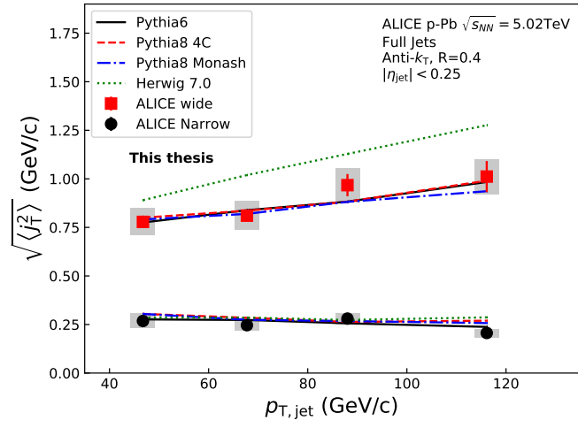
Figure 6.3: RMS values extracted from the fits are compared to Monte Carlo models. PYTHIA reproduces the data well for both the narrow and wide components. Herwig produces wider distributions.
