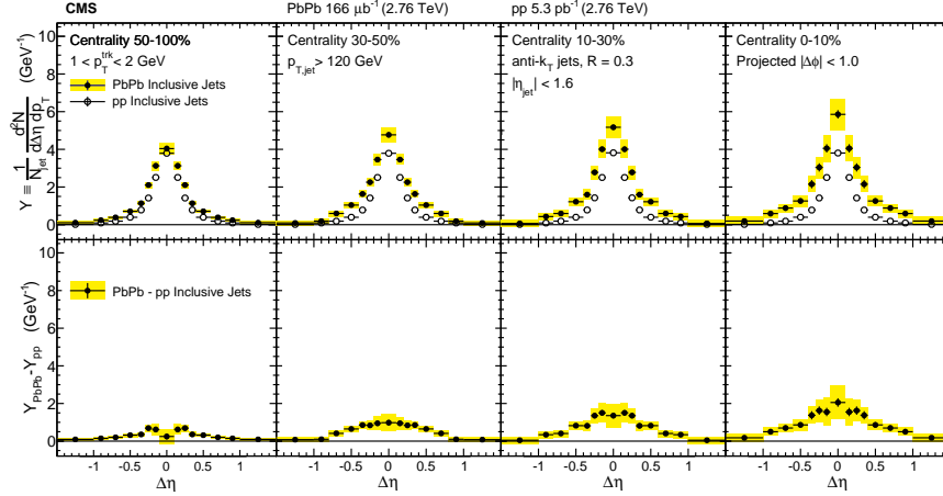
Figure 1.22: Measurement by CMS [164]. Symmetrized \Delta\eta distributions correlated with Pb–Pb and pp inclusive jets with p_T > 120 \text{ GeV}/c are shown in the top panels for tracks with 1 < p_T < 2 \text{ GeV}/c . The difference between per-jet yields in Pb–Pb and pp collisions is shown in the bottom panels. These measurements indicate that the jet is broadened and softened, as expected. The effect is stronger in more central collisions. \Delta\phi correlations have similar trends. Figure from [164]
