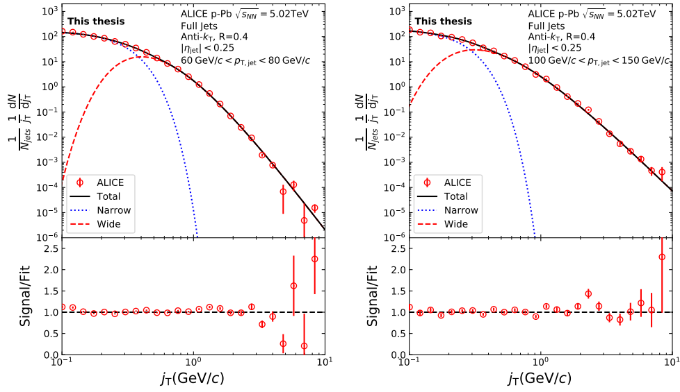
Figure 6.1: j_T signal distributions fitted with the two component model are shown in different jet p_T bins.
