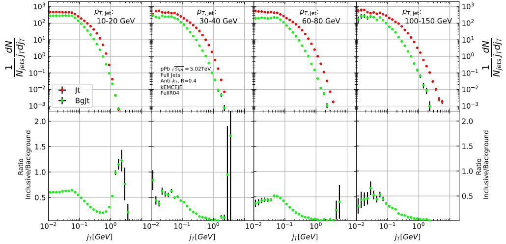
Figure 4.3: Inclusive j_T with background
