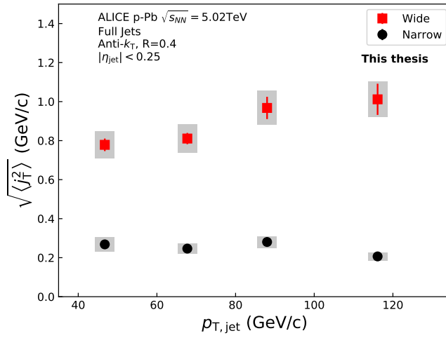
Figure 6.2: RMS values extracted from the fits are shown for the Gaussian (narrow) and inverse gamma (wide) components.
