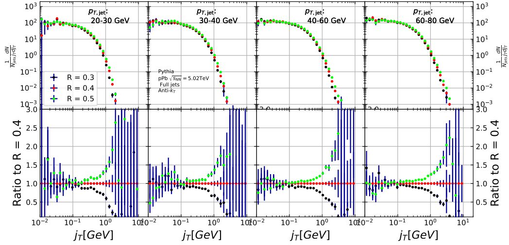
Figure 7.5: Effect of changing cone size on j_T distributions. The change is done both for the R parameter in the anti- k_T algorithm, and for the size of the cone where j_T is calculated.
