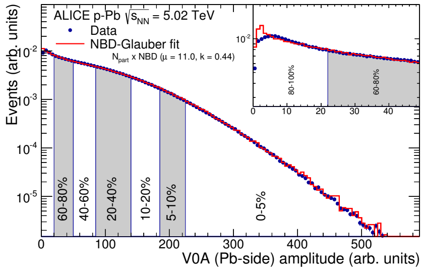
Figure 1.28: Distribution of the sum of amplitudes in p–Pb collisions in the V0A hodoscopes of ALICE (Pb-going side), as well as the NBD-Glauber fit. The vertical lines separate the centrality classes. Figure from [199].
