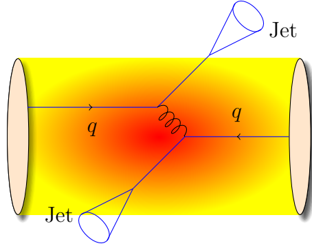
Figure 1.18: If hard scatterings happen in conjunction with QGP medium the produced jets must traverse the medium. Thus they are subject to interactions with the medium. Note that the dijet pair can be created anywhere within the medium volume and thus the two jets will have differing path lengths through the medium.
