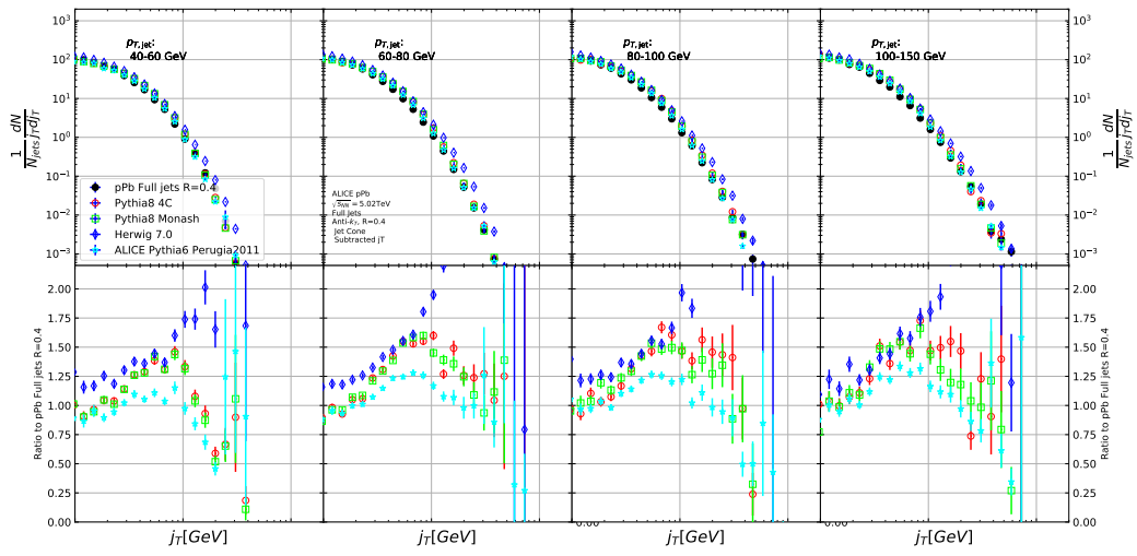
Figure B.2: Figure shows comparisons of j_T signals between ALICE data and various Monte Carlo simulations.
