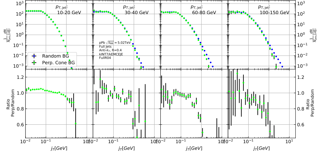
Figure 4.10: j_T background with two different methods
