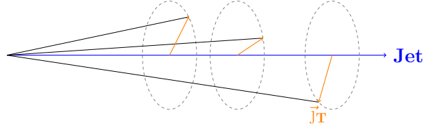
Figure 4.2: Illustration of \vec{j}_T . The jet fragmentation transverse momentum, \vec{j}_T , is defined as the momentum component of the track momentum, \vec{p}_{\text{track}} , that is transverse to the jet momentum, \vec{p}_{\text{jet}} .
