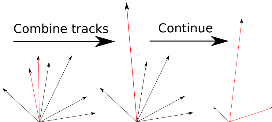
Figure 4.1: A simple example of the anti- k_T algorithm in progress. The red tracks in the leftmost figure are identified to have the smallest k_{T,i} in the event and are combined into the red track of the middle figure. As this continues the remaining tracks are added to this or other jets. One tracks was deemed to be isolated enough to be counted as a protojet by itself. Note that the rightmost figure is zoomed out.
