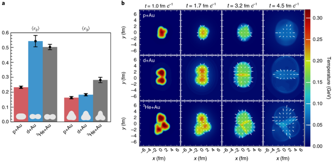
Figure 1.26: left : Eccentricities in different systems. right : Calculations of the initial energy density in small collision systems at RHIC and the resulting hydrodynamic evolution. This figure has been reprinted from [191] with kind permission from Springer Nature.
