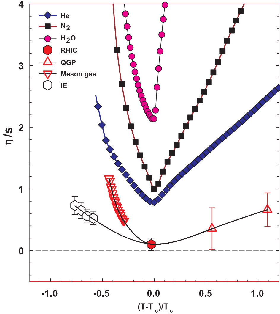
Figure 1.2: The figure shows \eta/s as a function of (T - T_c)/T_c for several substances as indicated. The lines are drawn to guide the eye. The \eta/s = 0.09 \pm 0.015 value at RHIC is estimated from Au–Au collisions at \sqrt{s_{NN}} = 200 GeV. The calculations assume a value T_c = 170 MeV for nuclear matter. This figure has been reprinted from [66] with kind permission from the American Physical Society.
