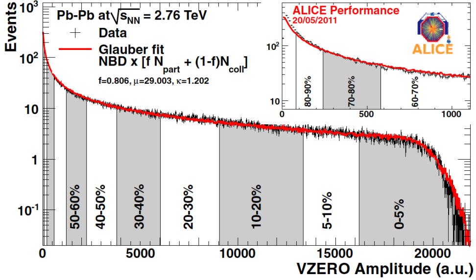
Figure 1.4: An illustration of the multiplicity distribution which is divided into centrality bins in ALICE measurements. The red line shows the fit of the Glauber calculation to the measurement. Figure from [79].
