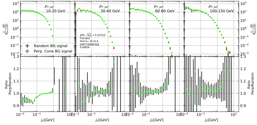
Figure 5.1: Comparison of the effect of background method on j_T signal
