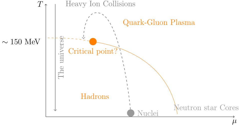
Figure 1.1: A schematic illustration of the phase diagram of QCD matter. The x -axis, showing the quark chemical potential \mu , represents the imbalance between quarks and antiquarks. Along the x -axis the temperature is zero. Along the vertical axis the temperature increases, which takes us through the crossover from a hadronic gas to quark-gluon plasma. With low \mu this is the regime explored by high-energy heavy-ion colliders and also the trajectory taken by the universe as it cooled after the Big Bang. The conditions in neutron stars correspond to the lower right corner, with low T and high \mu .
