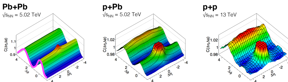
Figure 1.24: Two-particle correlation results in Pb–Pb , p–Pb , and pp collisions at the LHC [187]. This figure has been reprinted from [7] with kind permission from Annual Reviews.
