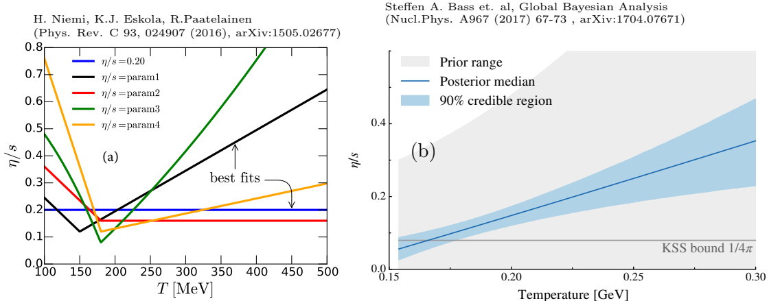
Figure 1.11: Temperature dependence of \eta/s . left : Different parametrisations of \eta/s(T) that have been tested in hydrodynamical simulations. right : Result of a global Bayesian analysis narrowing down the possible \eta/s(T) behaviour. These figures have been reprinted from [107] and [111] with kind permissions from the American Physical Society.
