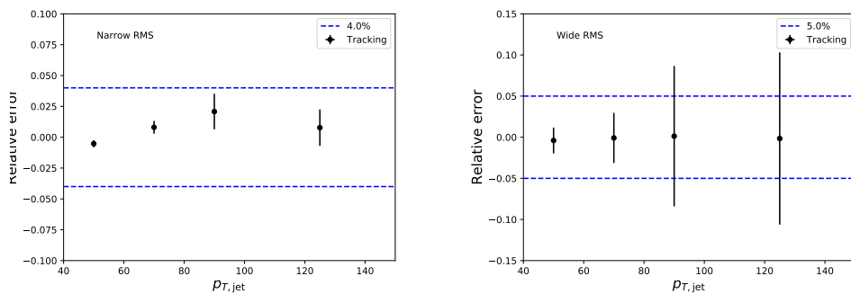
Figure 5.8: Relative systematic uncertainties resulting from uncertainty in tracking efficiency
