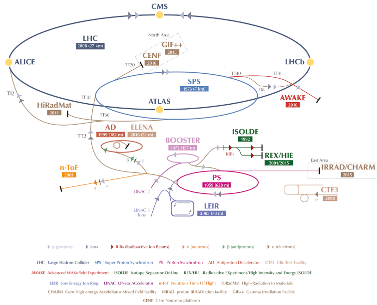
Figure 2.1: A schematic view of the accelerator complex at CERN. Before particles can be injected into the LHC they require a series of accelerators with increasing size. Until 2018 protons started their journey in LINAC2 (Linear Accelerator) and continue through the Booster, Proton Synchrotron (PS) and Super Proton Synchrotron (SPS). Between 2019 and 2020 LINAC2 will be replaced by LINAC4. Figure from [202].
