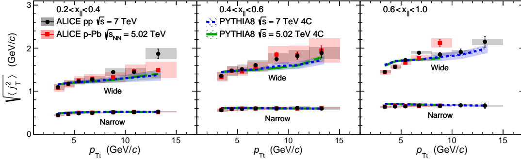
Figure 7.2: RMS values of the narrow and wide j_T components in the dihadron correlation analysis. Results from pp collisions at \sqrt{s} = 7 TeV (circular symbols) and from p-Pb collisions at \sqrt{s_{\text{NN}}} = 5.02 TeV (square symbols) are compared to PYTHIA 8 tune 4C simulations at \sqrt{s} = 7 TeV (short dashed line) and at \sqrt{s} = 5.02 TeV (long dashed line). Different panels correspond to different x_{\parallel} bins with 0.2 < x_{\parallel} < 0.4 on the left, 0.4 < x_{\parallel} < 0.6 in the middle, and 0.6 < x_{\parallel} < 1.0 on the right. The statistical errors are represented by bars and the systematic errors by boxes. Figure from [277].
