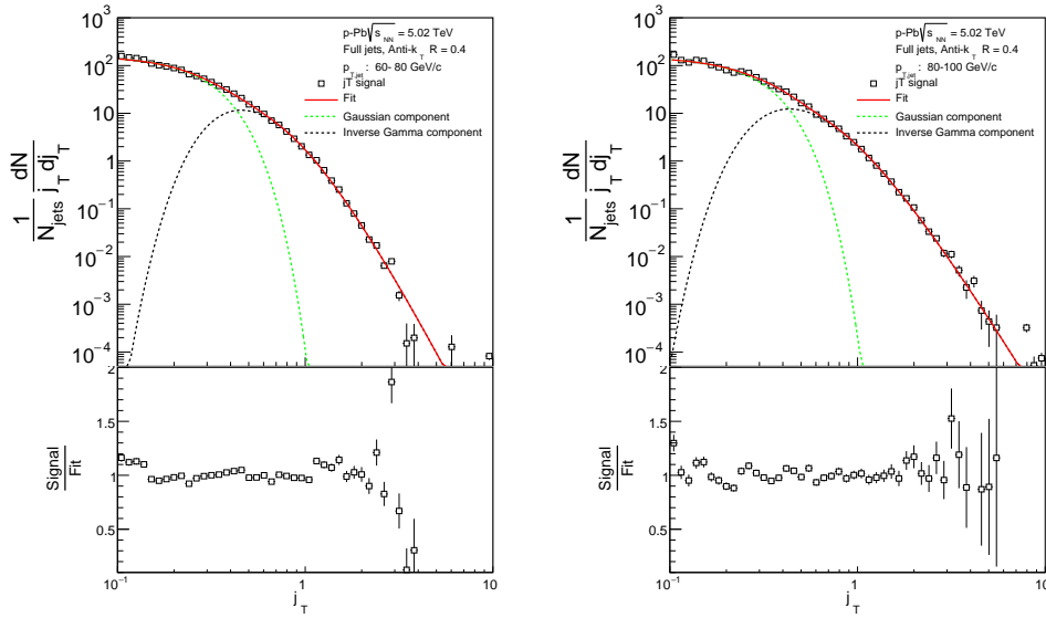
Figure 5.2: j_T signal with random background subtraction fits in different jet p_T bins
