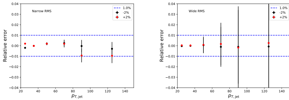
Figure 5.10: Relative systematic uncertainties resulting from cluster energy uncertainty.
