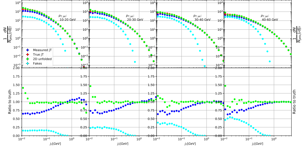
Figure 4.4: Results from unfolding in the pseudo-experiment Monte Carlo simulation
