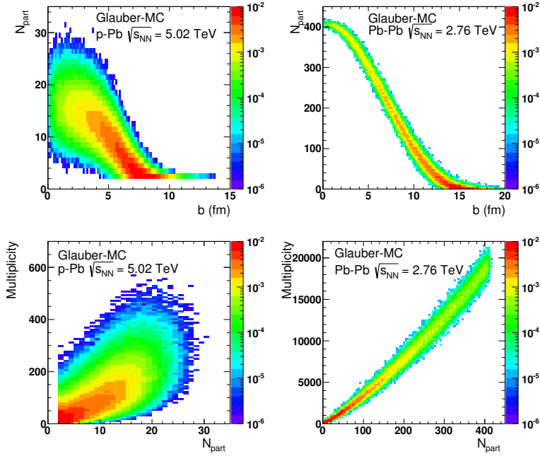
Figure 1.29: Top : Scatter plot of number of participating nucleons versus impact parameter; Bottom : Scatter plot of multiplicity versus the number of participating nucleons from the Glauber fit for V0A. The quantities are calculated with Glauber Monte Carlo simulations of p–Pb (left) and Pb–Pb (right) collisions. Figure from [199].
