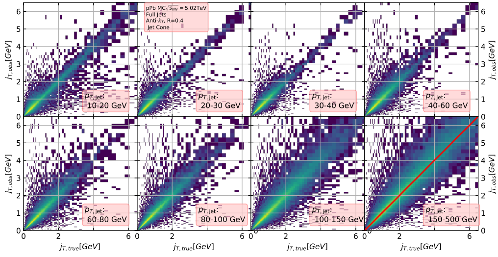
Figure 4.6: j_T Response matrices in individual p_{T,jet} bins
