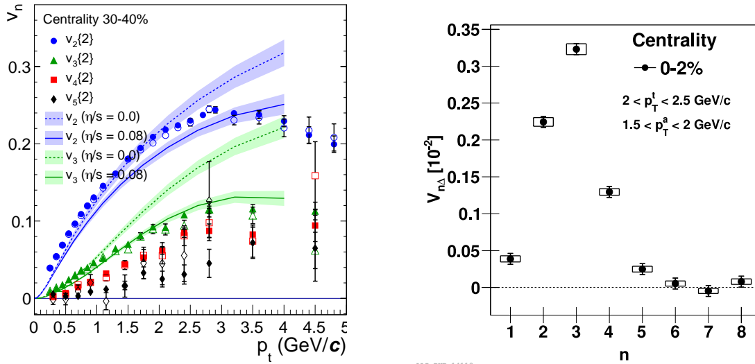
Figure 1.10: Flow measurements of higher harmonics. left : ALICE measurement of v_2 , v_3 , v_4 , v_5 as a function of transverse momentum. Two-particle correlations are used to obtain the harmonic coefficients. The full and open symbols are for different \Delta\eta separation between the particles ( \Delta\eta > 0.2 and \Delta\eta > 1.0 ). The observations are compared to hydrodynamic calculations [100] with varying values of the shear viscosity to entropy ratio \eta/s . Figure from [101]. right : Amplitude of v_n coefficients as a function of n for the 2% most central collisions as measured by ALICE. Figure from [102].
