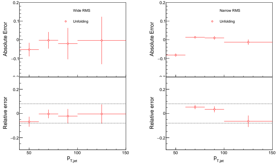
Figure 5.4: Differences between Bayesian and SVD unfolding in the resulting RMS values
