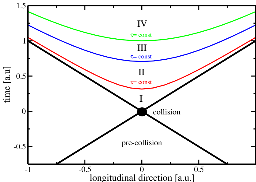
Figure 1.7: Schematic representation of a heavy-ion collision as a function of time and the longitudinal coordinate z . The various stages of the evolution are separated by hyperbolic curves which are defined by fixed proper time \tau = \sqrt{t^2 - z^2} . Figure from [90].
