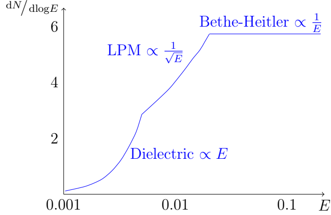
Figure 1.20: The expected bremsstrahlung spectrum for an electron propagating through material.
