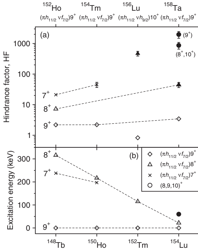
FIG. 4. (a) \alpha -decay hindrance factors from high-spin states of odd-odd N = 85 isotones to states in N = 83 daughter nuclei. The spins, parities, and configurations of the decaying states are shown on the upper axis with those of the populated states indicated in the inset of the lower panel (where assignments have been made). (b) The energies of the states populated in the daughter nuclei, indicated on the lower axis, relative to the 9^+ ground states. Error bars which lie within the symbols have been omitted and newly measured values for either hindrance factors (a) or level energies (b) are shown as full symbols. Points that are linked by dashed lines in the lower panel are sets of final states with the same configuration and those in the upper panel which also have the same initial state in the \alpha -decay process.
