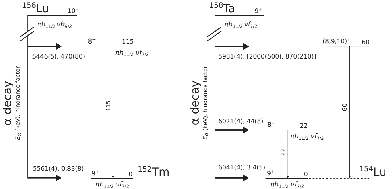
FIG. 1. Level schemes of ^{152}\text{Tm} and ^{154}\text{Lu} populated following the \alpha decays of ^{156}\text{Lu}(10^+) and ^{158}\text{Ta}(9^+) , respectively. The spins, parities, and energies of each level are given along with the energies of the transitions (in keV). For each \alpha decay the \alpha -particle energies and hindrance factors are given and the state populated is also indicated. The structures which have previously been assigned to states are shown (see text for details).
