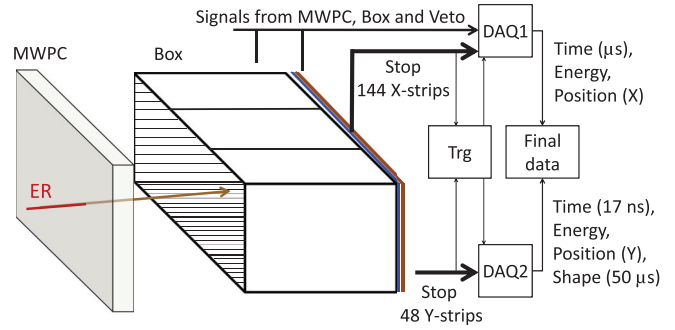
FIG. 2. Schematic illustrations of the focal plane detection setup of TASCA and the Combined ANalog and Digital (CANDI) data acquisition system coupled to the DSSD stop, box, veto, and MWPC detectors. Data acquisition (DAQ1 and DAQ2) was triggered (Trg) by both X and Y strip signals in ‘OR’ logical mode. For details, see text.
