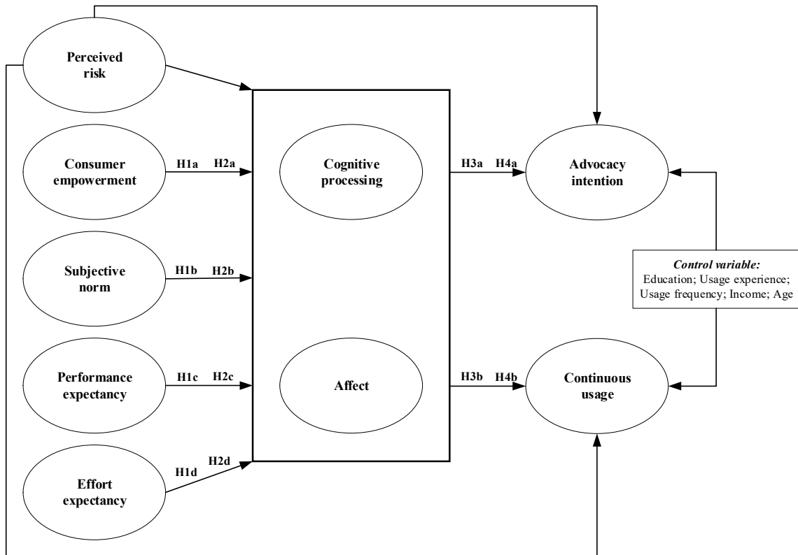
Figure 2 Conceptual model.
