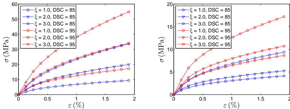
Figure 2: Stress-strain curves in the direction 1 (left) and the direction 2 (right) for the anisotropies \xi of 1, 2 and 3 with the dry solids contents (DSC) of 85% and 95%.
