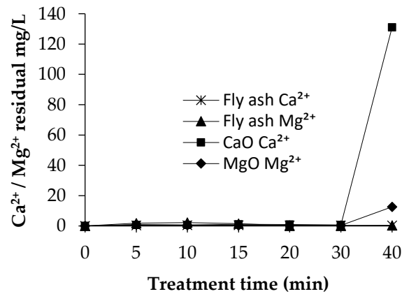
Figure 5. Atomic absorption spectroscopy (AAS) characterization of residual concentrations of \text{Ca}^{2+} and \text{Mg}^{2+} during the fly ash, CaO, and MgO experiments, at 20 °C.
