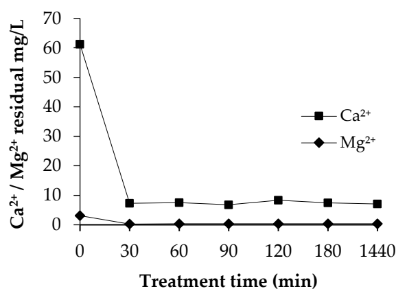
Figure 9. Inductively coupled plasma optical emission spectrometry (ICP-OES) characterization of the residual concentrations of Ca 2+ and Mg 2+ during the experiment, at 20 °C.
