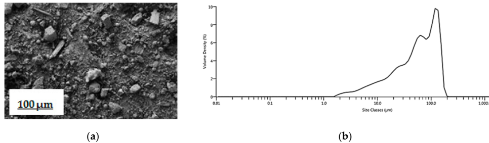
Figure 2. (a) FESEM image of untreated fly ash, 250 \times , the bar indicates 100 \mu\text{m} length.; (b) particle size distribution of fly ash.
