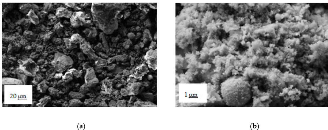
Figure 10. (a) SEM image of the solid precipitates in the authentic solution experiment, where the bar indicates 20 μm length; (b) SEM image of the solid precipitates in the authentic solution experiment, where the bar indicates 1 μm length.
