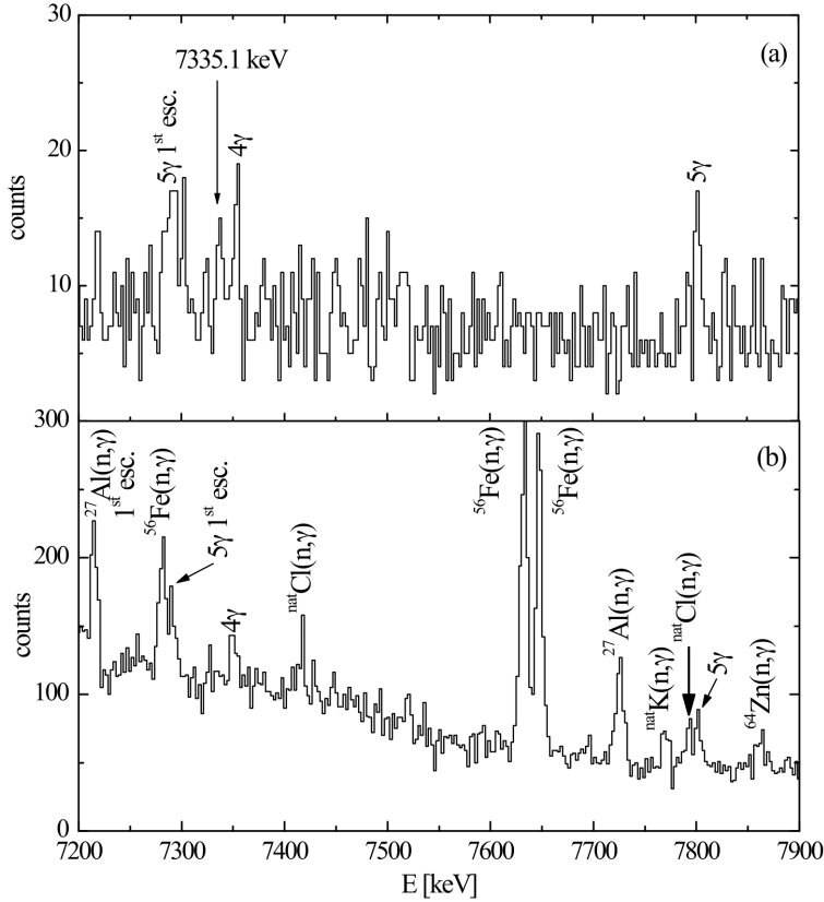
Fig. 2 The high energy part of the \gamma -spectrum from \beta -decay of ^{23}\text{Al} as reported in Ref. [16].
