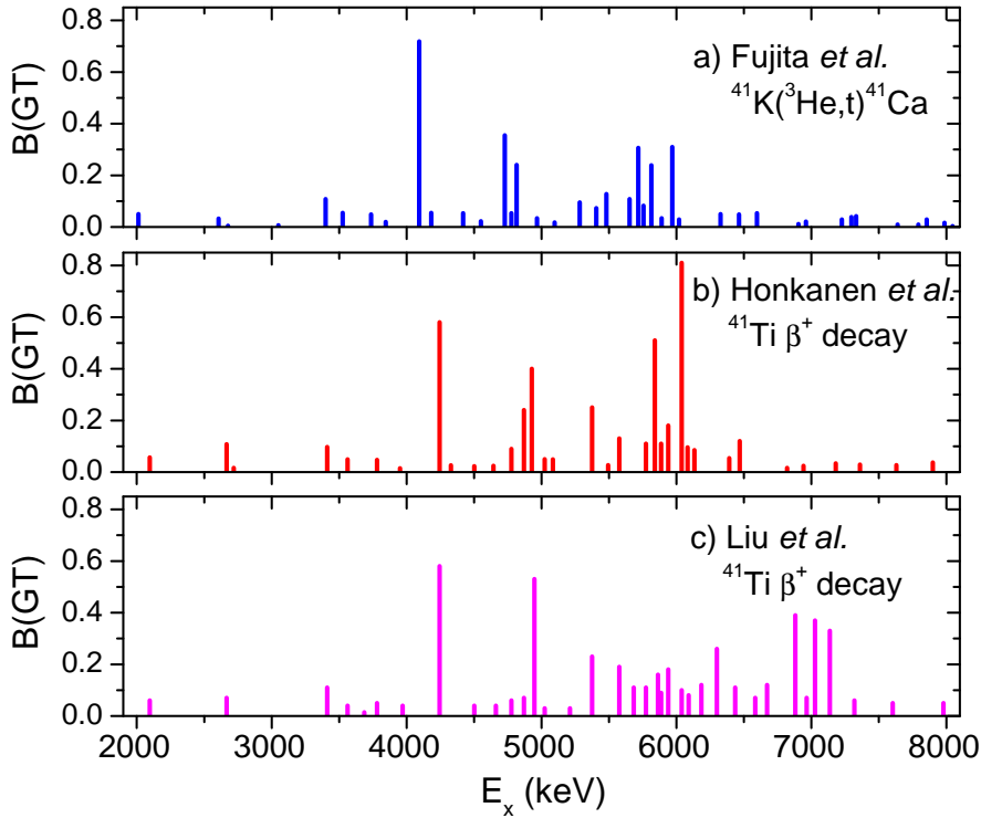
Fig. 4 Experimental B(GT) distributions for T_Z = \pm 3/2 \rightarrow T_Z = \pm 1/2 isospin mirror transitions from Refs. [1, 18, 65].
