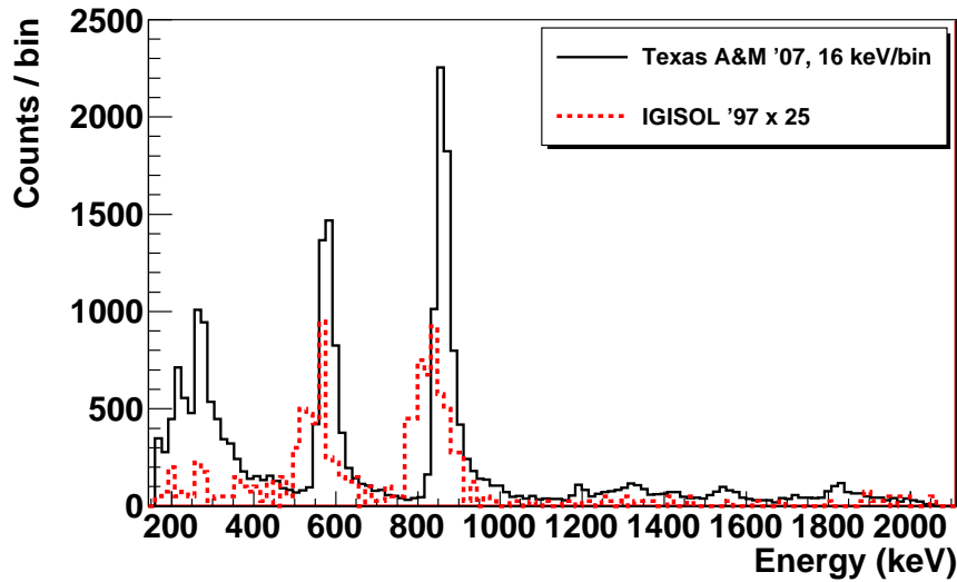
Fig. 3 Comparison of the proton spectra from IGISOL and Texas A&M. The IGISOL spectrum is multiplied \times 25 to scale with statistics of the Texas A&M experiment. Note that the IGISOL spectrum has its energy recorded as proton energy in lab, while the Texas A&M spectrum is the recorded total decay energy.
