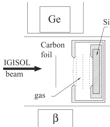
Fig. 1 Schematic presentation of the setup in the IGISOL central beam-line for ^{23}\text{Al} \beta -decay experiment reported in Refs. [16, 23]. The 40-keV beam was implanted into 40\ \mu\text{g}/\text{cm}^2 carbon foil surrounded by 37.5% HPGe detector, 1-mm-thick plastic \beta -detector and the \Delta E_{\text{gas}} - E_{\text{Si}} detector telescope.
