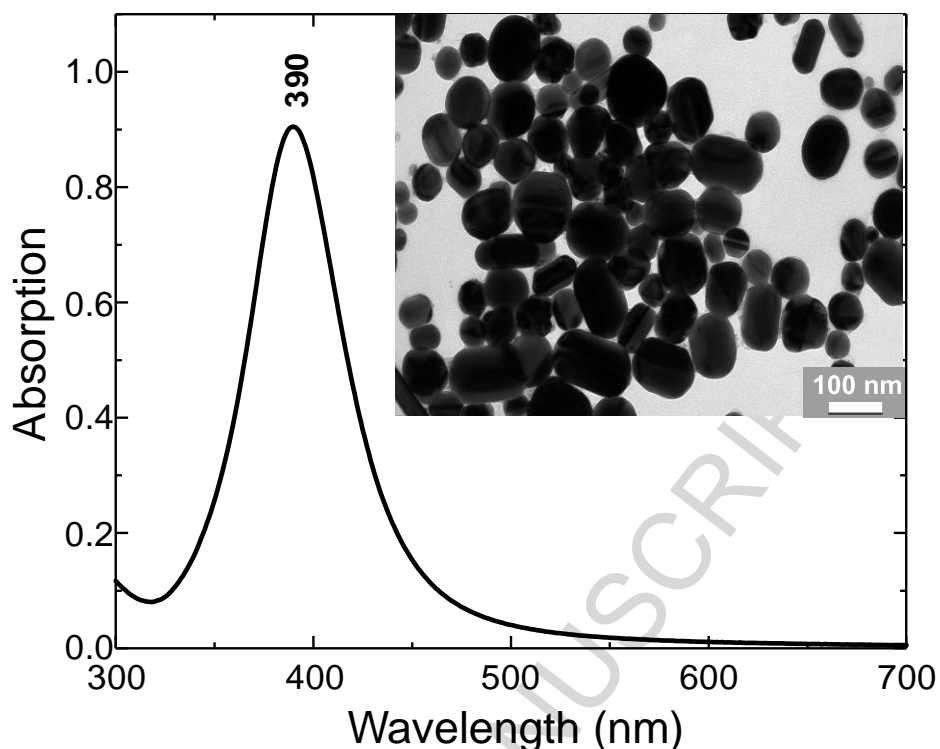
Figure 1. UV-Vis spectrum of aggregated silver nanoparticles. The spectrum shows a clear absorption band at 390 nm. The inset shows a high magnification transmission electron microscope image of a variety of structural features, i.e. hot-spots with plasmonic gap mode forming at the junctions of two or more Ag nanoparticles, that may be responsible for signal enhancement.
