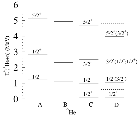
FIG. 4. Spectroscopy of low lying states in {}^9\text{He} . (a) Shell-model predictions from Ref. [2]. (b) Experimental result from Ref. [1]. (c) Modern shell-model calculations [6] with the WBT interaction of Warburton and Brown [21], shifted by 4.0 MeV (in this calculation {}^9\text{He} appeared to be unbound by 4.1 MeV). (d) Levels observed in this work, with the additional 1/2^+ level from Ref. [6]. Dashed lines correspond to the energy window of this experiment. Equation (2) was used to calculate excitation energies of {}^9\text{He} levels from the observed {}^9\text{Li}(T=5/2) resonances.
