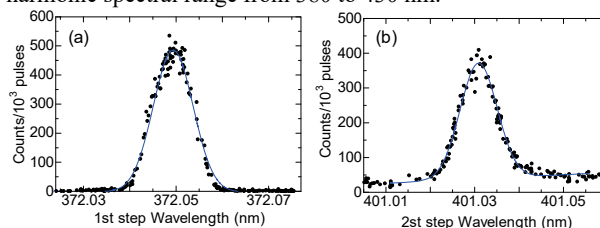
Figure 6. Resonance ionization spectra (a) 1 st step transition at 372.049 nm, (b) 2 nd step transition at 401.031 nm.
