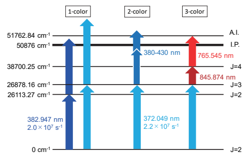
Figure 4. Resonance ionization schemes for Th used in this work. The number indicated below the wavelength is Einstein A coefficient of the transition.
