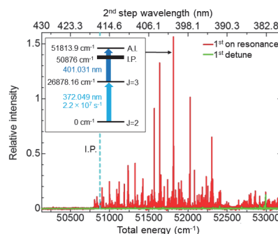
Figure 5. Results of wide wavelength scan in the second harmonic spectral range from 380 to 430 nm.
