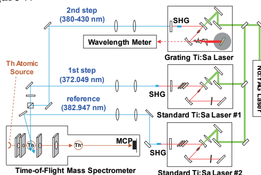
Figure 3. Experimental setup for investigation of two-color scheme for ionization of Th.
