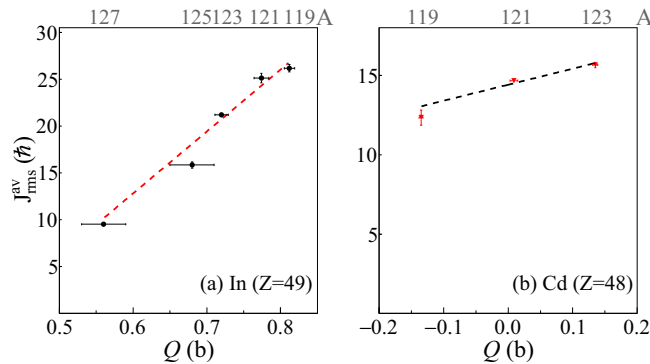
FIG. 4. Correlation between the electric quadrupole moments Q and the deduced J_{rms} values of the primary fission fragments for the isotopes of (a) In and of (b) Cd. The dashed lines represent the weighted least-squares fit.
