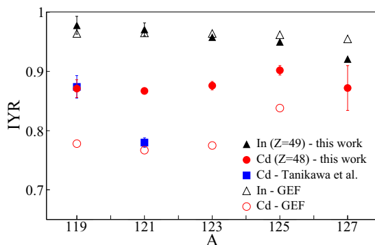
FIG. 3. The experimentally determined isomeric yield ratios for the isotopes of In and Cd as measured in this work by employing the PI-ICR technique. The data are compared with data available in the literature [72], and with results from calculations performed with the GEF model [70,71]. The error bars in the experimental results are smaller than the data points, whenever they are not visible in the figure.
