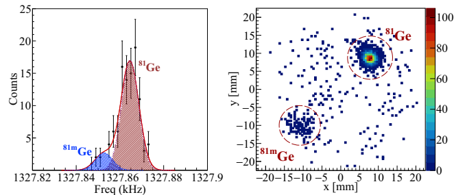
FIG. 1. The case of ^{81}\text{Ge} , observed with the sideband cooling technique (left) and with the PI-ICR technique (right). The dashed circles are used to guide the eye.
