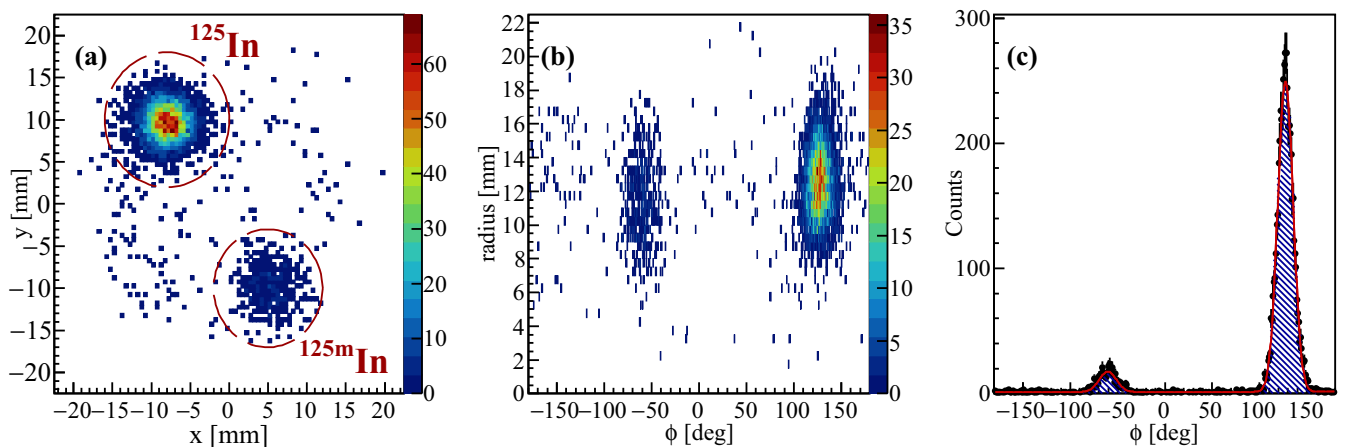
FIG. 2. (a) A typical histogram showing the position of the two states of ^{125}\text{In} , separated by 180^\circ . The next two panels illustrate the analysis procedure followed in this work. In panel (b), the position of the ions is converted to polar coordinates. In panel (c), the yield of each state is determined from Gaussian fitting on the \phi projection. The dashed circles are used to guide the eye.
