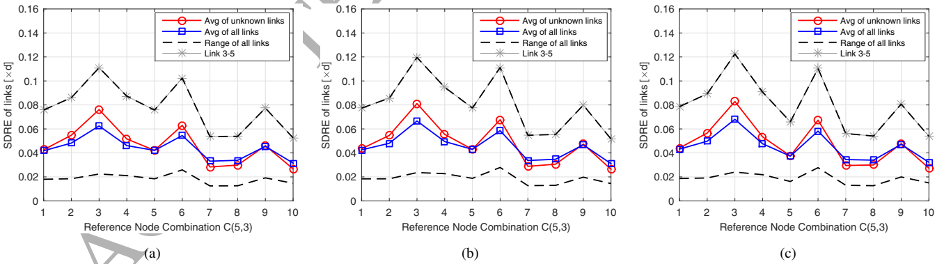
Figure 9: SDRE of the links vs. reference node combinations (see Table 6) using the PLE estimation technique (a) Weighted Mean PLE 1, (b) Weighted LSE PLE 1, (c) SSE Minimization 1. A measurement period of one week (July 21–27, 2014).
