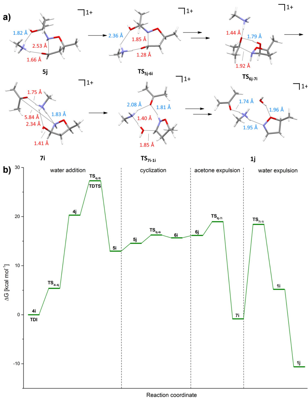
Figure 4. a) Optimized structures for 5j , TS 5j-6i , TS 6j-7i , 7i , TS 7i-1i , 1j in last three steps (all optimized structures are given in supporting info, Fig. S5). b) Calculated Gibbs free energies for acetone oxime model (listed also in Tab. S3).
