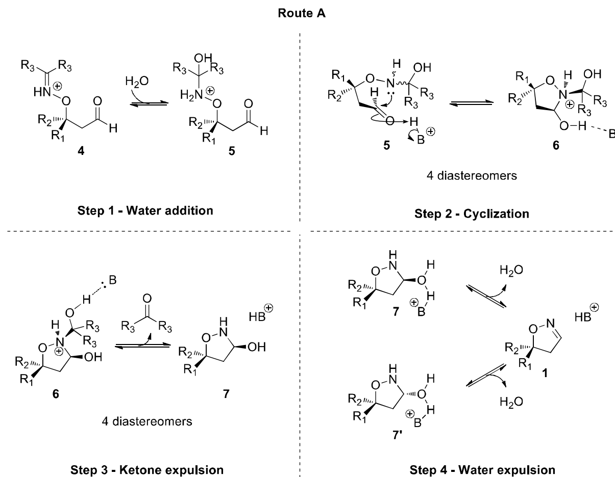
Scheme 2. Proposed reaction route for isoxazoline formation from conjugate addition product 4 .
