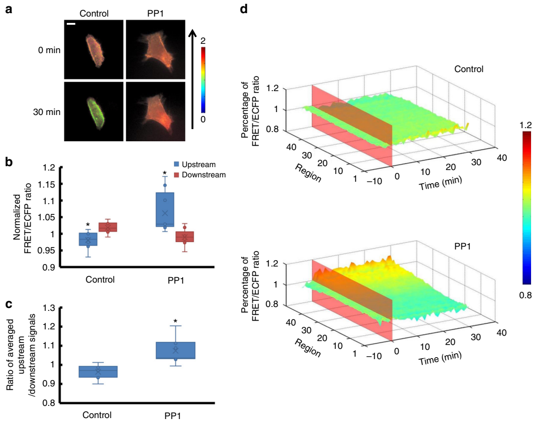
Fig. 7 The affinity of RhoGDI \alpha and Rho GTPases under shear stress is affected by Src. a Living cell images of Lyn-sl-RhoGDI \alpha biosensor under 20 dyn cm -2 of shear stress with 50 mmol per L of the Src inhibitor PP1 ( n = 7 ). The scale bar is 10 \mu m. b The FRET/ECFP ratio comparison of upstream to downstream, after normalization. c Averaged upstream/downstream ratio for the control group and the PP1 group. The asterisk denotes that there is an obvious difference between upstream and downstream. d Binding degree distribution of RhoGDI \alpha and Rho GTPases is enhanced at upstream regions along the flow direction when Src is inhibited. The FRET ratio percentage of each region overall is normalized before shear stress application. The asterisk denotes that there is an obvious difference compared to the control group
