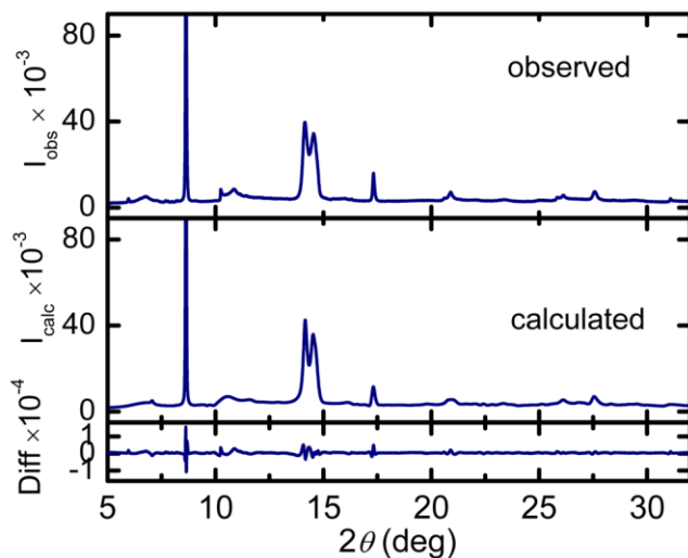
Figure 4. Observed and calculated PXRD pattern for cis -cofacial 4-pyDTDA ( \lambda = 0.825925 \text{ \AA} ).
