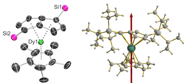
Fig. 1 Left: Thermal ellipsoid representation (50% probability) of the molecular structure of \mathbf{1}_{Dy} (with H-atoms and ^1Pr groups omitted for clarity). Right: the principal axis of the g -tensor in the ground Kramers doublet of \mathbf{1}_{Dy} .
