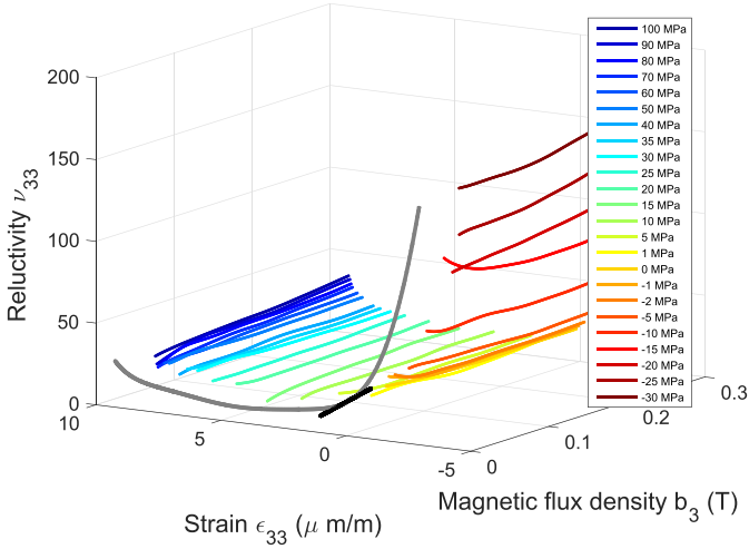
Fig. 7. Reluctivity component \nu_{33} = h_3/b_3 is plotted as a function of \epsilon_{33} and b_3 . For numerical reasons, we left out points for which b_3 < 0.05 T. The data points b_3 > 0.3 T are left out, because we are in search of linear model with respect to b_3 . We observe that within chosen limits the reluctivity \nu_{33} depends only on \epsilon_{33} , not b_3 . The gray curve is a polynomial of the order 8 fit to the (\epsilon_{33}, \nu_{33}) -data. The black line is the linear part of the polynomial at \epsilon_{33} = 0 . We can approximate \nu_{33} = \nu_\epsilon \epsilon_{33} + \nu_M when |\epsilon_{33}| < 0.5 \mu\text{m/m} .
