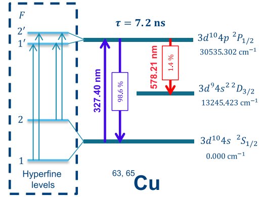
FIG. 5. Atomic levels and their hyperfine splitting (not to scale) in the stable ^{63,65}\text{Cu} isotopes.
