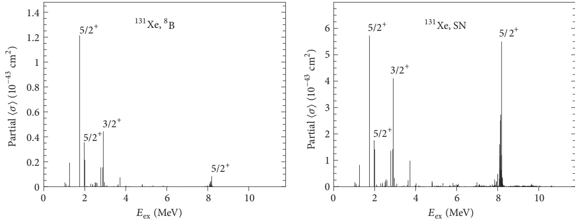
FIGURE 7: Contributions to the inelastic scattering averaged cross section arising from various final states of ^{131}\text{Xe} at energies E_{\text{ex}} . Results are shown for {}^8\text{B} solar neutrinos (left panel) and supernova electron neutrinos (right panel). In both panels cross sections are given in units of 10^{-43} \text{ cm}^2 .
