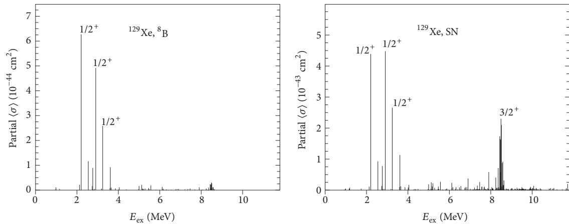
FIGURE 8: Contributions to the inelastic scattering averaged cross section arising from various final states of ^{129}\text{Xe} at energies E_{\text{ex}} . Results are shown for {}^8\text{B} solar neutrinos (left panel) and supernova electron neutrinos (right panel). Cross sections are given in units of 10^{-44} \text{ cm}^2 for solar neutrinos and 10^{-43} \text{ cm}^2 for supernova neutrinos.
