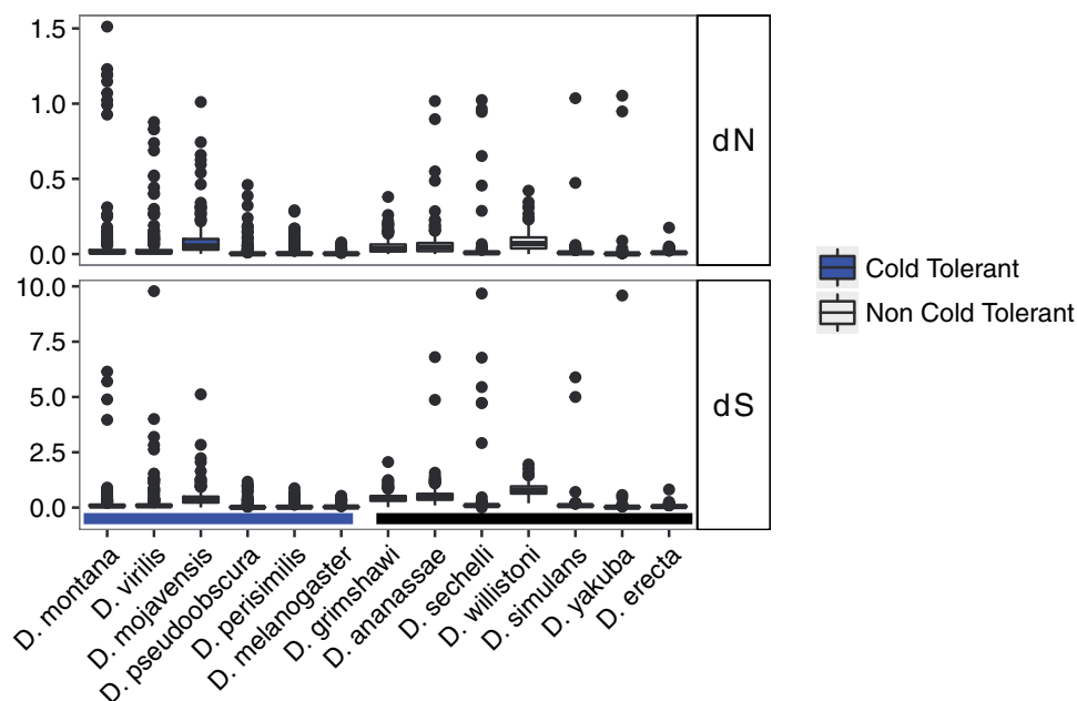
Fig. 2. —Distributions of dN and dS estimates for each of the 250 genes from 13 Drosophila species with significant differences in \omega between cold-tolerant and non-cold-tolerant species.
