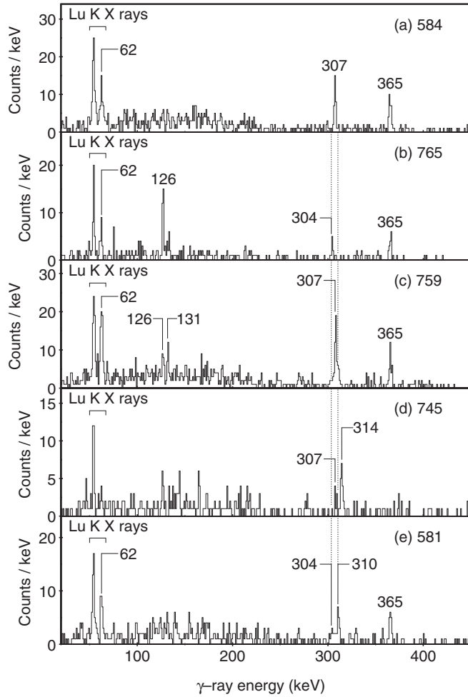
FIG. 3. Energy spectra of \gamma rays observed in the planar Ge detector in coincidence with (a) 584-, (b) 765-, (c) 759-, (d) 745-, and (e) 581-keV \gamma rays in the clover Ge detectors. All \gamma rays were required to occur within 0.5 \mu\text{s} of the implantation of an ion into the DSSDs and be followed in the same DSSD pixel by a 5565-keV \alpha decay of ^{156}\text{Lu} within 576 ms. No background has been subtracted from the coincidence matrix. The dotted lines indicate the positions of the 304- and 310-keV \gamma -ray peaks. Peaks are labeled with their energies in keV.
