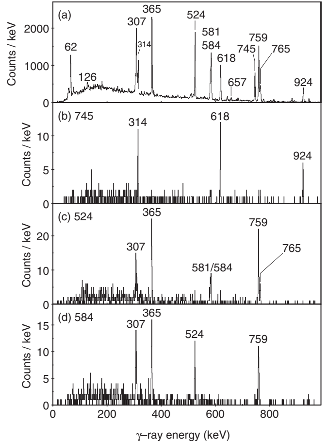
FIG. 1. Energy spectra of \gamma rays observed in the clover Ge detectors deployed at the focal plane of RITU. All \gamma rays were required to be detected within 0.5\ \mu\text{s} of the implantation of an ion into the DSSDs and be followed in the same DSSD pixel by a 5565-keV ^{156}\text{Lu} \alpha decay within 576 ms. (a) Single energy spectrum of delayed ^{156}\text{Lu} \gamma rays observed in the clover Ge detectors. Energy spectra of \gamma rays observed in the clover Ge detectors in coincidence with 745-, 524-, and 584-keV \gamma rays in other crystals of the clover Ge detectors are shown in panels (b), (c), and (d), respectively. No background has been subtracted from the coincidence matrix. Peaks are labeled with their energies in keV.
