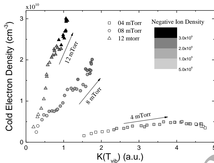
Figure 17. Color-coded negative ion density on the plane of electron density versus vibrational temperature. Instead of the actual vibrational temperature, the rate coefficient K(T_{\text{vib}}) is used.
