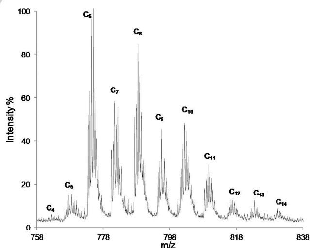
Figure 5. ESI-MS profile for the competition experiment of guests ranging from C_4 to C_{14} (1 eq. of each guest) in the presence of 1 equivalent of cage 1a\cdot Cu . Each isotopic pattern labelled with C_n represents the inclusion complex C_n@1a\cdot Cu
