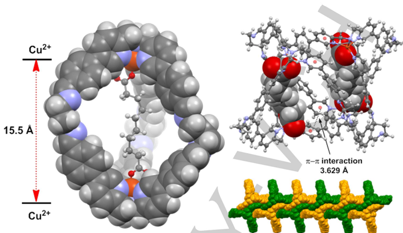
Figure 4. (a) X-ray crystal structure of C_{10}@1b\cdot Cu in CPK model displaying the entrapment of sebacic acid C_{10} (ball & stick model) inside the cage. (b) Section of 3-D packing to highlight \pi - \pi stabilization of C_{10}@1b\cdot Cu cage entities. The sebacic acid C_{10} is shown in CPK model. (c) 1-D polymer formation.
